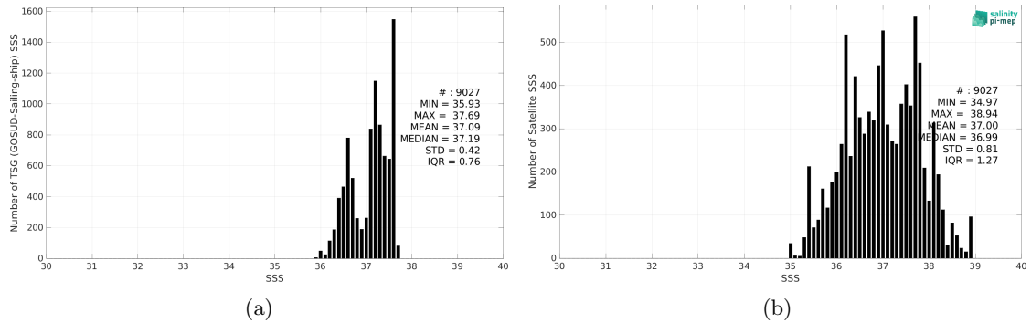
Figure 2: Histograms of SSS from TSG (GOSUD-Sailing-ship) (a) and SMOS SSS L2Q v331 - No FLAG (CMEMS-CATDS-CPDC) (b) considering all match-up pairs per bins of 0.1 over the SPURS 1 Pi-MEP region and for the full satellite product period.
