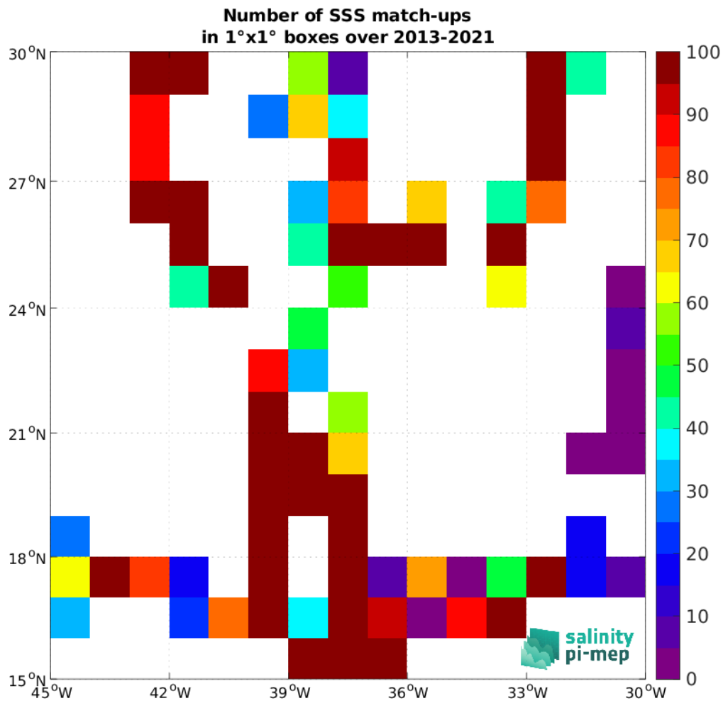
Figure 4: Number of SSS match-ups between TSG (GOSUD-Sailing-ship) SSS and the SMOS SSS L2Q v331 - No FLAG (CMEMS-CATDS-CPDC) SSS product for the SPURS 1 Pi-MEP region over 1^\circ \times 1^\circ boxes and for the full satellite product period.
