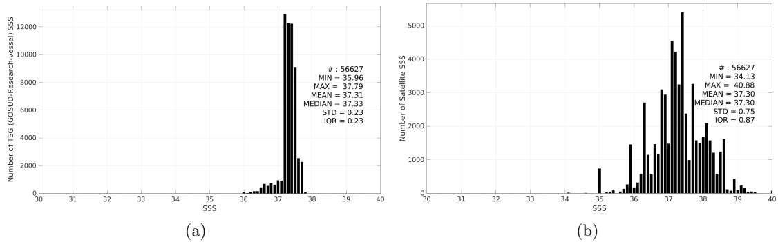
Figure 3: Histograms of SSS from TSG (GOSUD-Research-vessel) (a) and SMOS SSS L2Q v331 - No FLAG (CMEMS-CATDS-CPDC) (b) considering all match-up pairs per bins of 0.1 over the SPURS 1 Pi-MEP region and for the full satellite product period.
