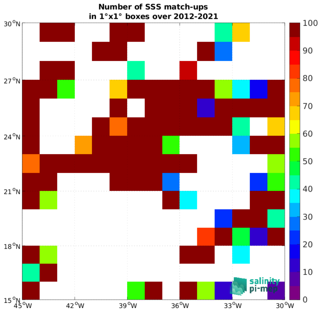
Figure 5: Number of SSS match-ups between TSG (GOSUD-Research-vessel) SSS and the SMOS SSS L2Q v331 - No FLAG (CMEMS-CATDS-CPDC) SSS product for the SPURS 1 Pi-MEP region over 1^\circ \times 1^\circ boxes and for the full satellite product period.
