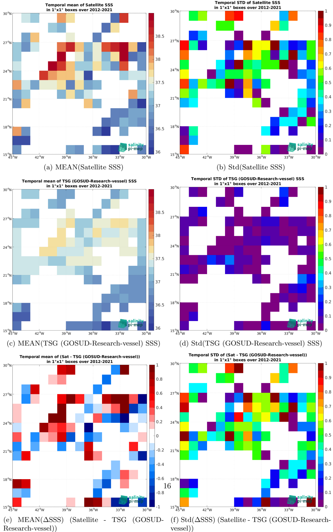
Figure 7: Temporal mean (left) and Std (right) of SSS from SMOS SSS L2Q v331 - No FLAG (CMEMS-CATDS-CPDC) (top), TSG (GOSUD-Research-vessel) (middle), and of \Delta SSS (Satellite - TSG (GOSUD-Research-vessel)). Only match-up pairs are used to generate these maps.
