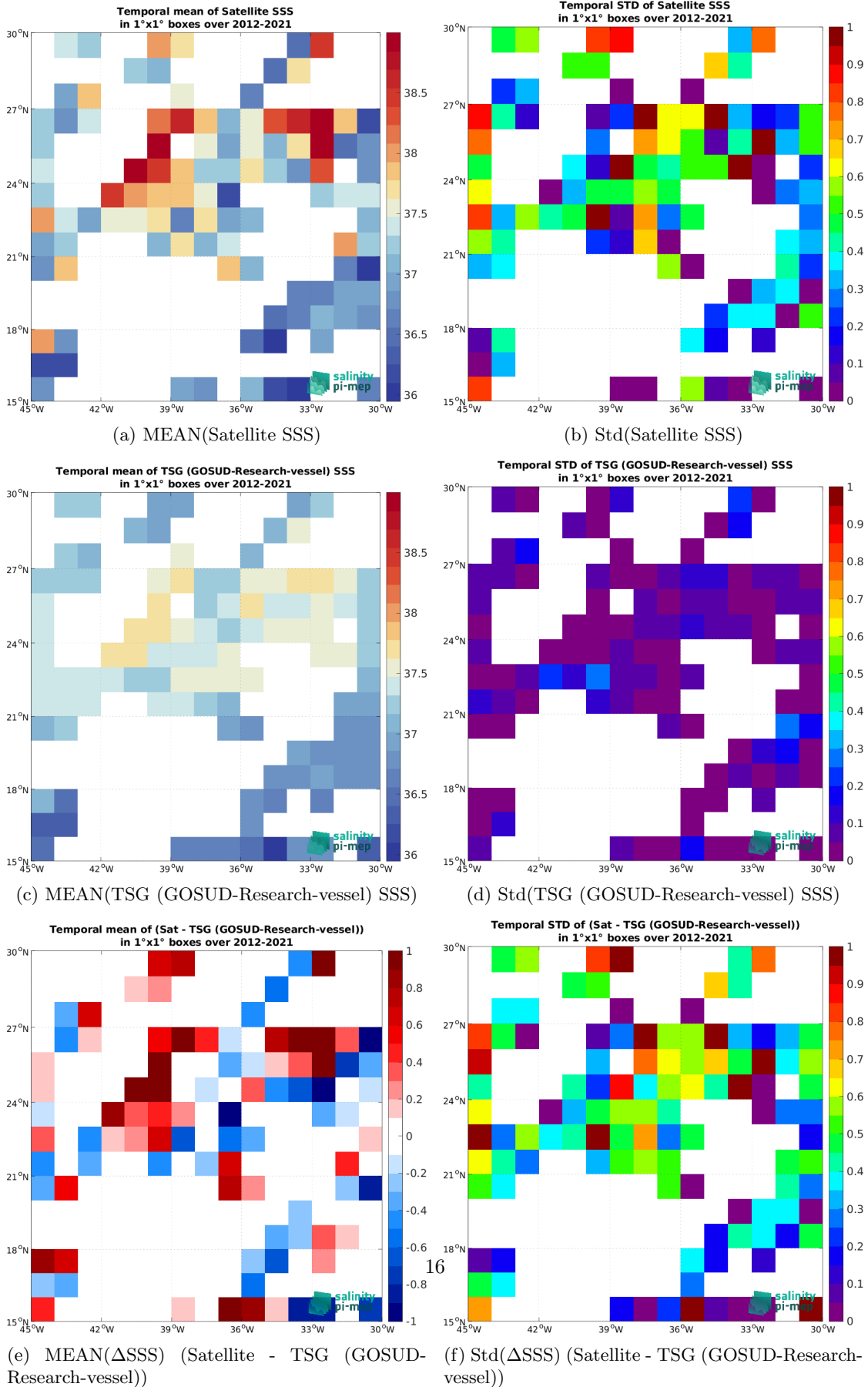
Figure 6: Temporal mean (left) and Std (right) of SSS from SMOS SSS L2Q v331 - No FLAG (CMEMS-CATDS-CPDC) (top), TSG (GOSUD-Research-vessel) (middle), and of \Delta SSS (Satellite - TSG (GOSUD-Research-vessel)). Only match-up pairs are used to generate these maps.
