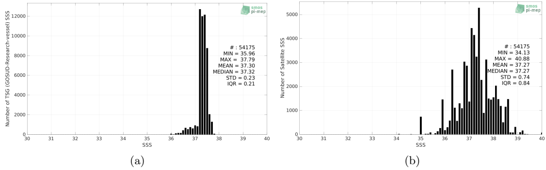
Figure 2: Histograms of SSS from TSG (GOSUD-Research-vessel) (a) and SMOS SSS L2Q v331 - No FLAG (CMEMS-CATDS-CPDC) (b) considering all match-up pairs per bins of 0.1 over the SPURS 1 Pi-MEP region and for the full satellite product period.
