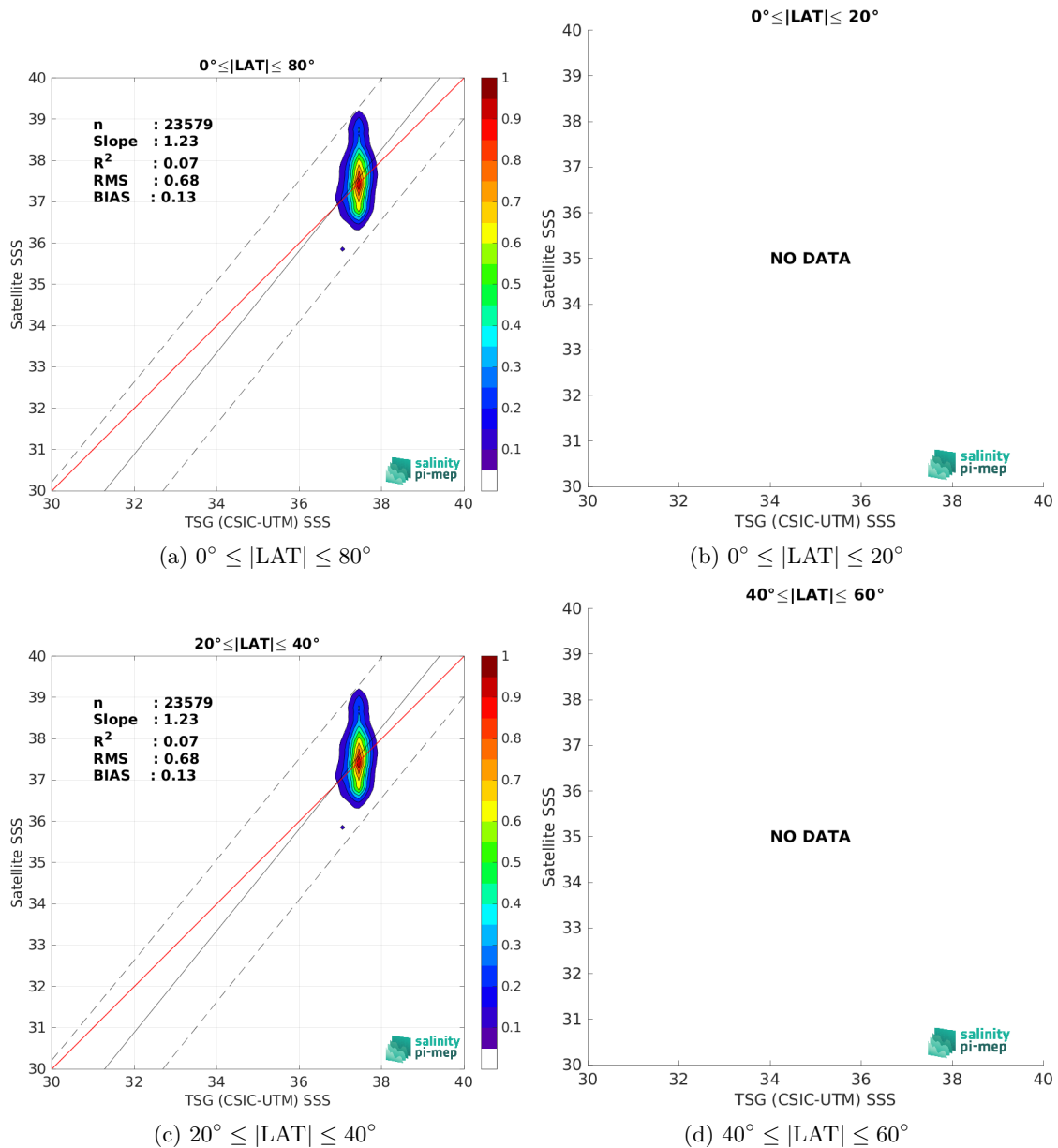
Figure 10: Contour maps of the concentration of SMOS SSS L2Q v331 - No FLAG (CMEMS-CATDS-CPDC) SSS (y-axis) versus TSG (CSIC-UTM) SSS (x-axis) at match-up pairs for different latitude bands. For each plot, the red line shows x=y . The black thin and dashed lines indicate a linear fit through the data cloud and the \pm 95\% confidence levels, respectively. The number match-up pairs n , the slope and R^2 coefficient of the linear fit, the root mean square (RMS) and the mean bias between satellite and in situ data are indicated for each latitude band in each plots.
