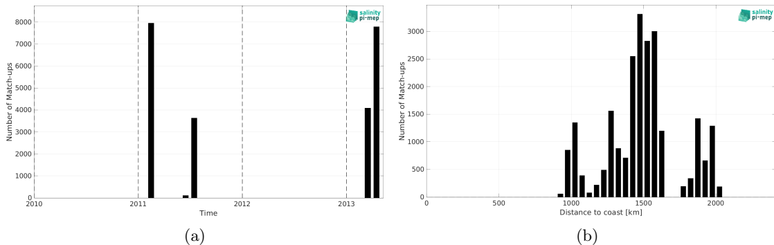
Figure 2: Number of match-ups between TSG (CSIC-UTM) and SMOS SSS L2Q v331 - No FLAG (CMEMS-CATDS-CPDC) SSS as a function of time (a) and as function of the distance to coast (b) over the SPURS 1 Pi-MEP region and for the full satellite product period.
