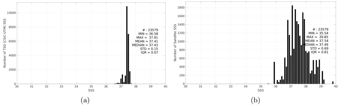
Figure 3: Histograms of SSS from TSG (CSIC-UTM) (a) and SMOS SSS L2Q v331 - No FLAG (CMEMS-CATDS-CPDC) (b) considering all match-up pairs per bins of 0.1 over the SPURS 1 Pi-MEP region and for the full satellite product period.
