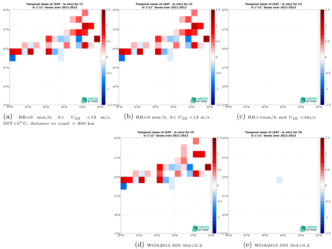
Figure 14: Temporal mean gridded over spatial boxes of size 1^\circ \times 1^\circ of \Delta SSS (SMOS SSS L2Q v331 - No FLAG (CMEMS-CATDS-CPDC) - TSG (CSIC-UTM)) for 5 different subdatasets corresponding to: RR=0 mm/h, 3 < U_{10} < 12 m/s, SST > 5^\circ\text{C} , distance to coast > 800 km (a), RR=0 mm/h, 3 < U_{10} < 12 m/s (b), RR > 1 mm/h and U_{10} < 4 m/s (c), WOA2013 SSS Std < 0.2 (d), WOA2013 SSS Std > 0.2 (e).
