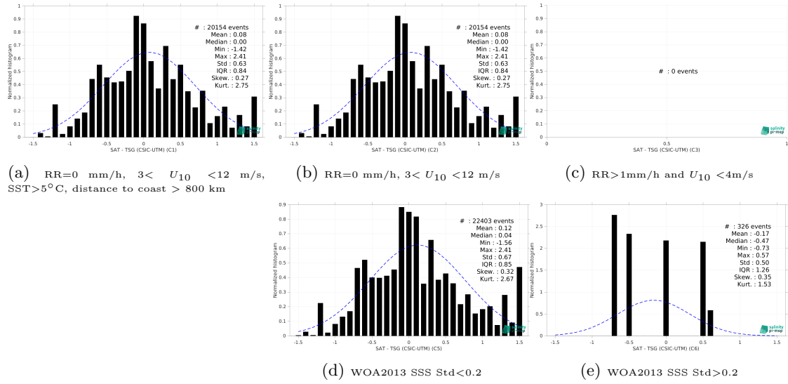
Figure 15: Normalized histogram of \Delta SSS (SMOS SSS L2Q v331 - No FLAG (CMEMS-CATDS-CPDC) - TSG (CSIC-UTM)) for 5 different subdatasets corresponding to: RR=0 mm/h, 3 < U_{10} < 12 m/s, SST>5°C, distance to coast > 800 km (a), RR=0 mm/h, 3 < U_{10} < 12 m/s (b), RR>1mm/h and U_{10} < 4 m/s (c), WOA2013 SSS Std<0.2 (d), WOA2013 SSS Std>0.2 (e).
