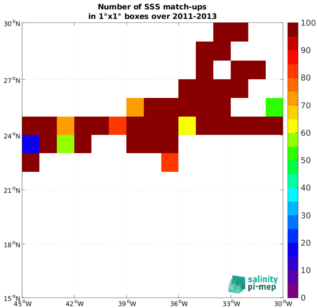
Figure 5: Number of SSS match-ups between TSG (CSIC-UTM) SSS and the SMOS SSS L2Q v331 - No FLAG (CMEMS-CATDS-CPDC) SSS product for the SPURS 1 Pi-MEP region over 1^\circ \times 1^\circ boxes and for the full satellite product period.
