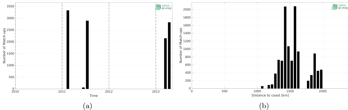
Figure 1: Number of match-ups between TSG (CSIC-UTM) and SMOS SSS L2Q v331 - No FLAG (CMEMS-CATDS-CPDC) SSS as a function of time (a) and as function of the distance to coast (b) over the SPURS 1 Pi-MEP region and for the full satellite product period.
