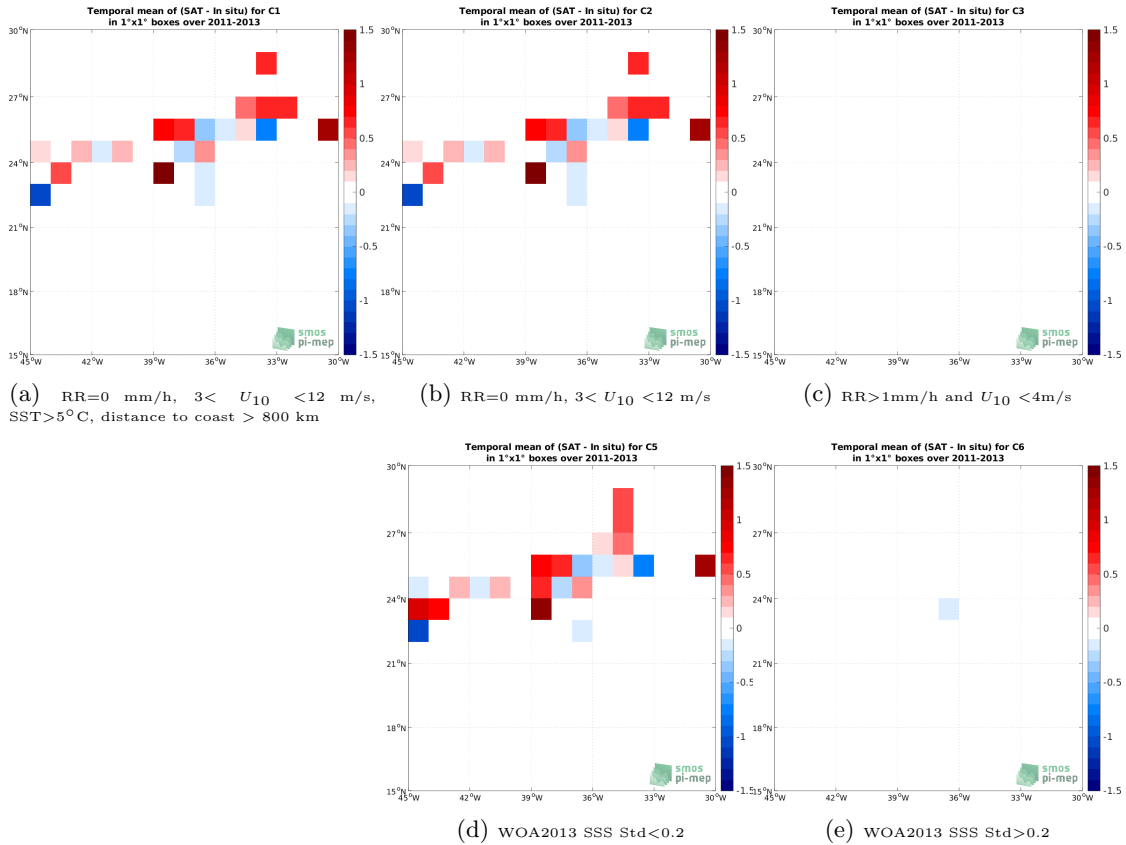
Figure 12: Temporal mean gridded over spatial boxes of size 1^{\circ}\times 1^{\circ} of \Delta\text{SSS} (SMOS SSS L2Q v331 - No FLAG (CMEMS-CATDS-CPDC) - TSG (CSIC-UTM)) for 5 different subdatasets corresponding to:RR=0 mm/h, 3 < U_{10} < 12 m/s, SST >5^{\circ}\text{C} , distance to coast > 800 km (a), RR=0 mm/h, 3 < U_{10} < 12 m/s (b), RR >1 mm/h and U_{10} < 4 m/s (c), WOA2013 SSS Std <0.2 (d), WOA2013 SSS Std >0.2 (e).
