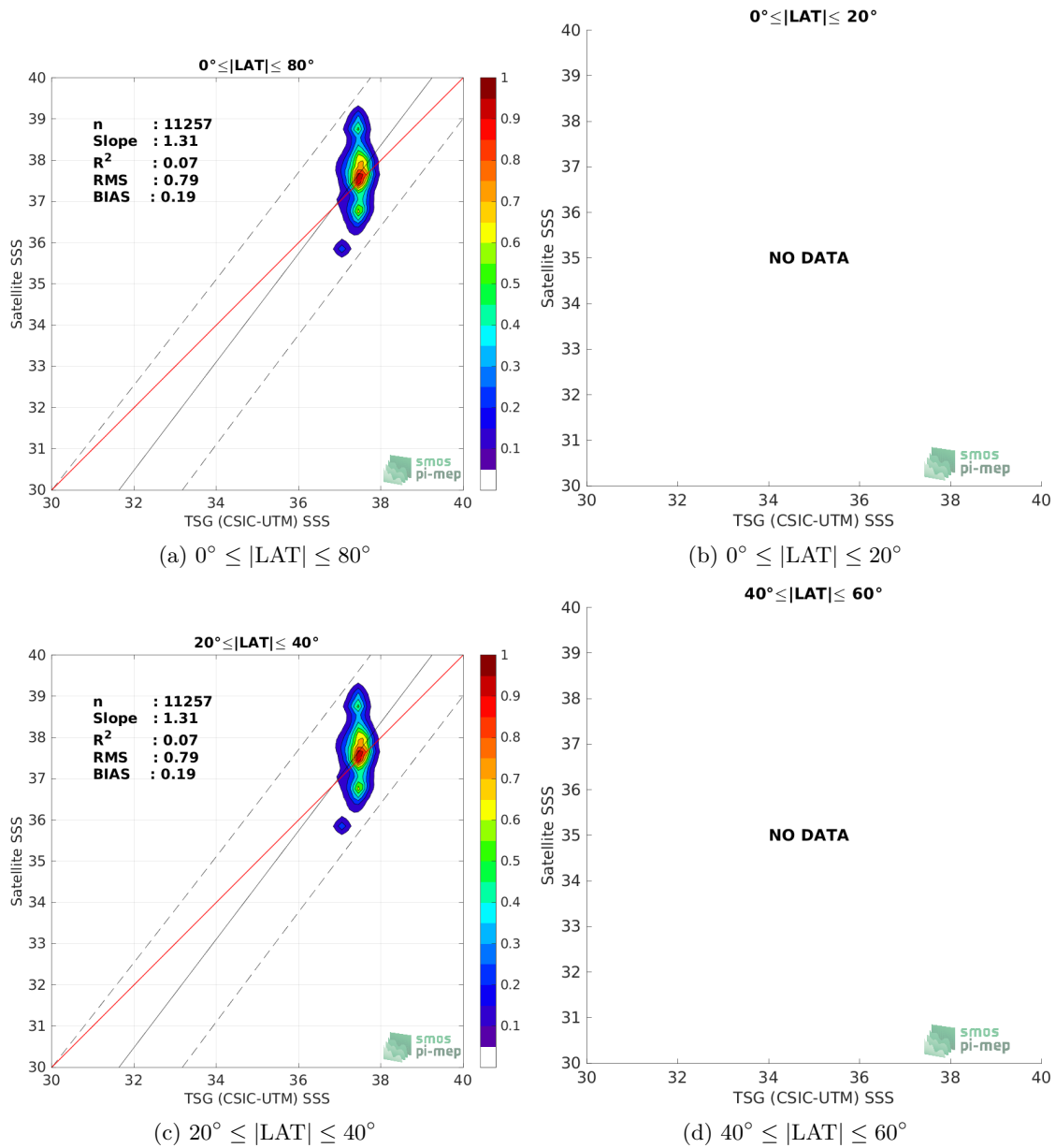
Figure 9: Contour maps of the concentration of SMOS SSS L2Q v331 - No FLAG (CMEMS-CATDS-CPDC) SSS (y-axis) versus TSG (CSIC-UTM) SSS (x-axis) at match-up pairs for different latitude bands. For each plot, the red line shows x=y . The black thin and dashed lines indicate a linear fit through the data cloud and the \pm 95\% confidence levels, respectively. The number match-up pairs n , the slope and R^2 coefficient of the linear fit, the root mean square (RMS) and the mean bias between satellite and in situ data are indicated for each latitude band in each plots.
