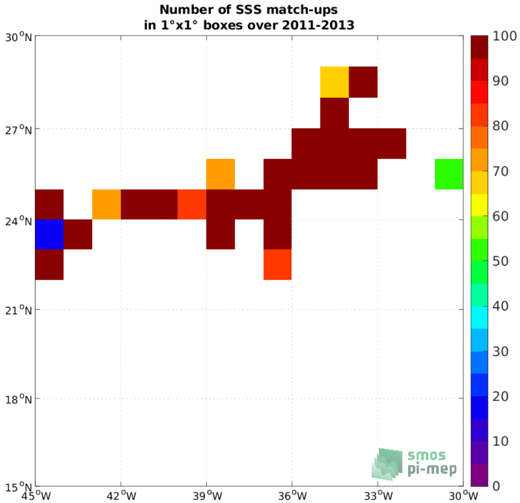
Figure 4: Number of SSS match-ups between TSG (CSIC-UTM) SSS and the SMOS SSS L2Q v331 - No FLAG (CMEMS-CATDS-CPDC) SSS product for the SPURS 1 Pi-MEP region over 1^\circ \times 1^\circ boxes and for the full satellite product period.
