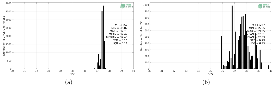
Figure 2: Histograms of SSS from TSG (CSIC-UTM) (a) and SMOS SSS L2Q v331 - No FLAG (CMEMS-CATDS-CPDC) (b) considering all match-up pairs per bins of 0.1 over the SPURS 1 Pi-MEP region and for the full satellite product period.
