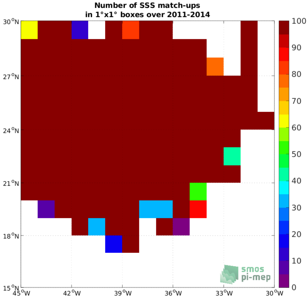
Figure 3: Number of SSS match-ups between Surface drifters SSS and the SMOS SSS L2Q v331 - No FLAG (CMEMS-CATDS-CPDC) SSS product for the SPURS 1 Pi-MEP region over 1°x1° boxes and for the full satellite product period.
