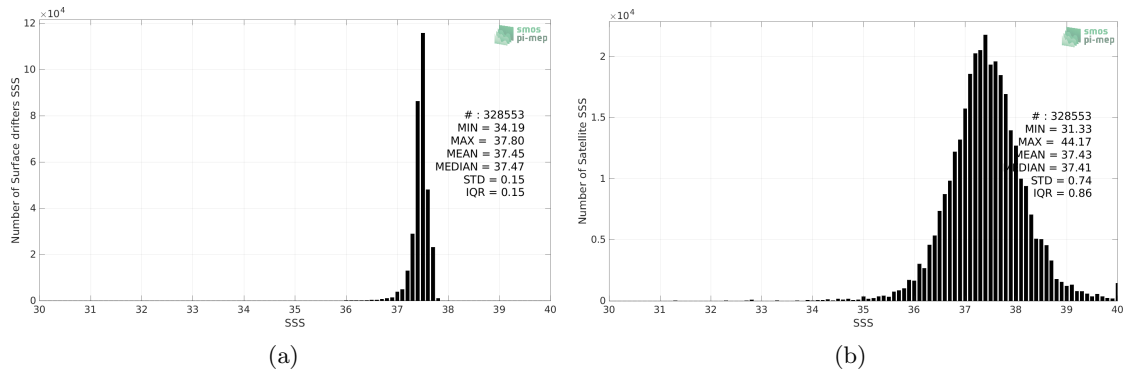
Figure 2: Histograms of SSS from Surface drifters (a) and SMOS SSS L2Q v331 - No FLAG (CMEMS-CATDS-CPDC) (b) considering all match-up pairs per bins of 0.1 over the SPURS 1 Pi-MEP region and for the full satellite product period.
