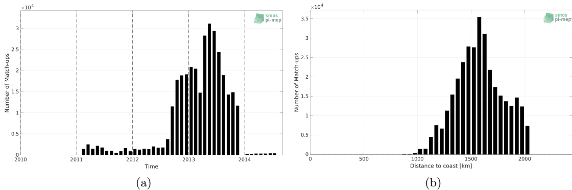
Figure 1: Number of match-ups between Surface drifters and SMOS SSS L2Q v331 - No FLAG (CMEMS-CATDS-CPDC) SSS as a function of time (a) and as function of the distance to coast (b) over the SPURS 1 Pi-MEP region and for the full satellite product period.
