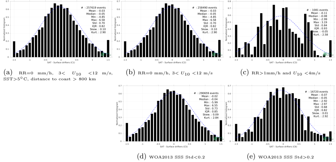
Figure 12: Normalized histogram of \Delta SSS (SMOS SSS L2Q v331 - No FLAG (CMEMS-CATDS-CPDC) - Surface drifters) for 5 different subdatasets corresponding to: RR=0 mm/h, 3 < U_{10} < 12 m/s, SST>5°C, distance to coast > 800 km (a), RR=0 mm/h, 3 < U_{10} < 12 m/s (b), RR>1mm/h and U_{10} < 4 m/s (c), WOA2013 SSS Std<0.2 (d), WOA2013 SSS Std>0.2 (e).
