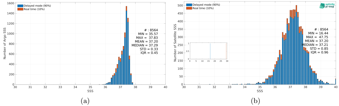
Figure 3: Histograms of SSS from Argo (a) and SMOS SSS L2Q v331 - No FLAG (CMEMS-CATDS-CPDC) (b) considering all match-up pairs per bins of 0.1 over the SPURS 1 Pi-MEP region and for the full satellite product period.
