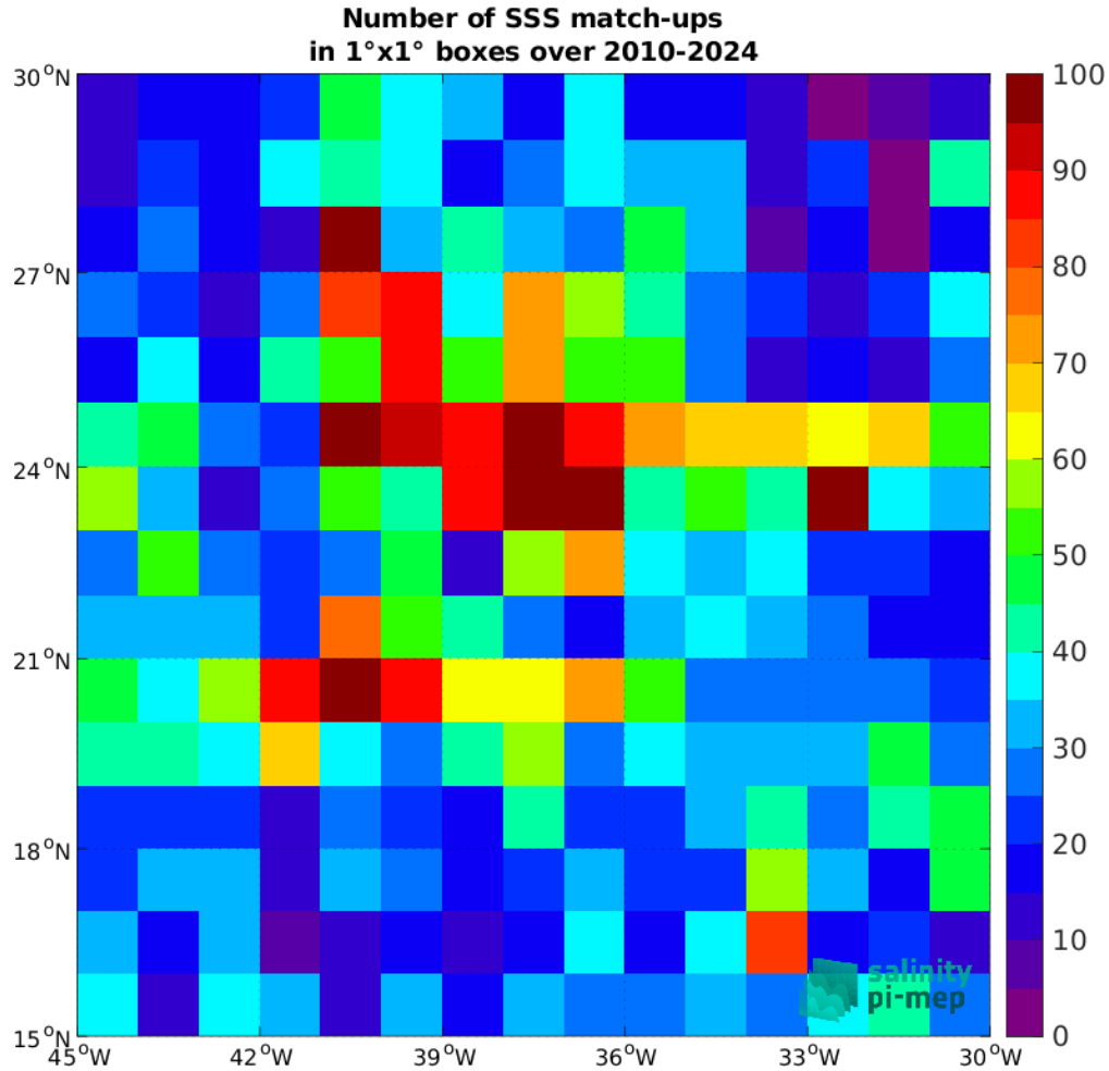
Figure 5: Number of SSS match-ups between Argo SSS and the SMOS SSS L2Q v331 - No FLAG (CMEMS-CATDS-CPDC) SSS product for the SPURS 1 Pi-MEP region over 1^\circ \times 1^\circ boxes and for the full satellite product period.
