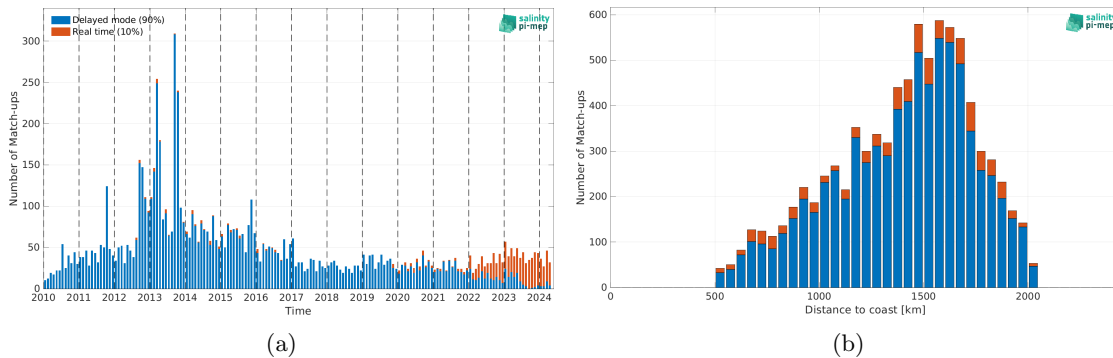
Figure 2: Number of match-ups between Argo and SMOS SSS L2Q v331 - No FLAG (CMEMS-CATDS-CPDC) SSS as a function of time (a) and as function of the distance to coast (b) over the SPURS 1 Pi-MEP region and for the full satellite product period.
