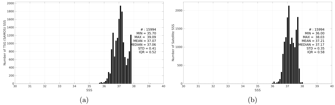
Figure 3: Histograms of SSS from TSG (SAMOS) (a) and SMOS SSS L3 v9 - 9 Days (CATDS-CEC-LOCEAN) (b) considering all match-up pairs per bins of 0.1 over the SPURS 1 Pi-MEP region and for the full satellite product period.
