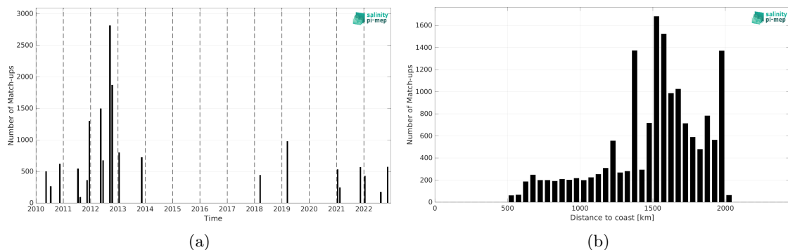
Figure 2: Number of match-ups between TSG (SAMOS) and SMOS SSS L3 v9 - 9 Days (CATDS-CEC-LOCEAN) SSS as a function of time (a) and as function of the distance to coast (b) over the SPURS 1 Pi-MEP region and for the full satellite product period.
