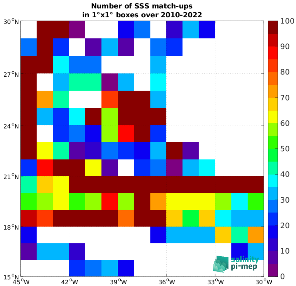
Figure 4: Number of SSS match-ups between TSG (SAMOS) SSS and the SMOS SSS L3 v9 - 9 Days (CATDS-CEC-LOCEAN) SSS product for the SPURS 1 Pi-MEP region over 1°x1° boxes and for the full satellite product period.
