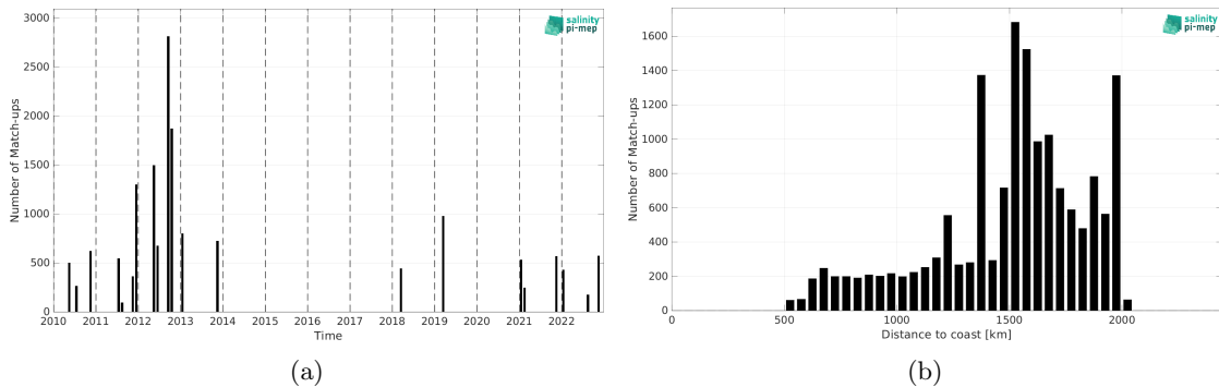
Figure 1: Number of match-ups between TSG (SAMOS) and SMOS SSS L3 v9 - 9 Days (CATDS-CEC-LOCEAN) SSS as a function of time (a) and as function of the distance to coast (b) over the SPURS 1 Pi-MEP region and for the full satellite product period.
