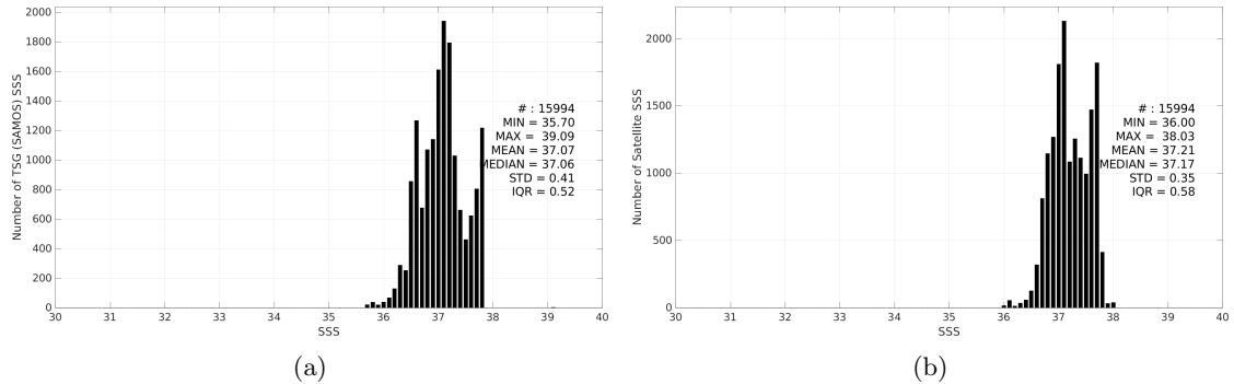
Figure 2: Histograms of SSS from TSG (SAMOS) (a) and SMOS SSS L3 v9 - 9 Days (CATDS-CEC-LOCEAN) (b) considering all match-up pairs per bins of 0.1 over the SPURS 1 Pi-MEP region and for the full satellite product period.
