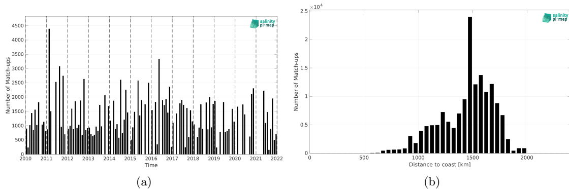
Figure 1: Number of match-ups between TSG (LEGOS-DM) and SMOS SSS L3 v9 - 9 Days (CATDS-CEC-LOCEAN) SSS as a function of time (a) and as function of the distance to coast (b) over the SPURS 1 Pi-MEP region and for the full satellite product period.
