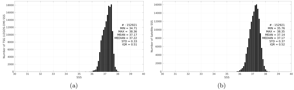
Figure 2: Histograms of SSS from TSG (LEGOS-DM) (a) and SMOS SSS L3 v9 - 9 Days (CATDS-CEC-LOCEAN) (b) considering all match-up pairs per bins of 0.1 over the SPURS 1 Pi-MEP region and for the full satellite product period.
