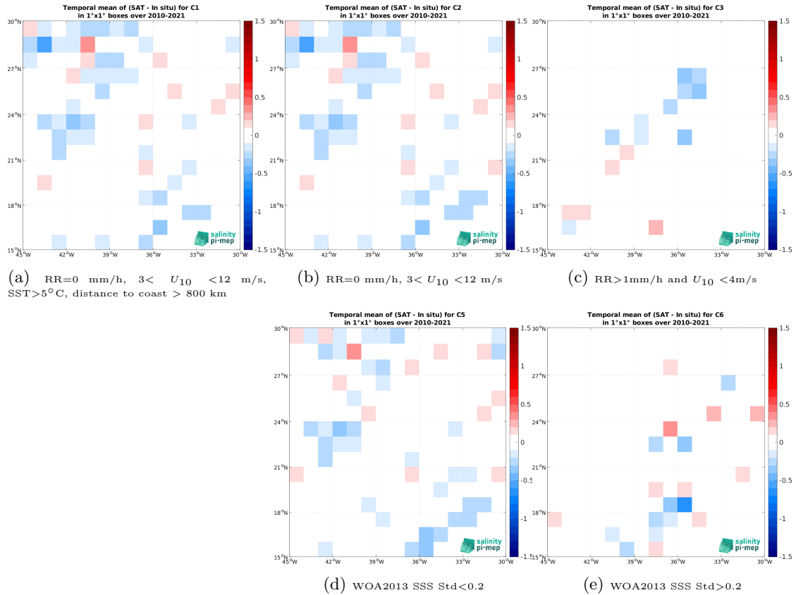
Figure 12: Temporal mean gridded over spatial boxes of size 1^{\circ}\times 1^{\circ} of \Delta\text{SSS} (SMOS SSS L3 v9 - 9 Days (CATDS-CEC-LOCEAN) - TSG (LEGOS-DM)) for 5 different subdatasets corresponding to:RR=0 mm/h, 3 < U_{10} < 12 m/s, SST >5^{\circ}\text{C} , distance to coast > 800 km (a), RR=0 mm/h, 3 < U_{10} < 12 m/s (b), RR >1 mm/h and U_{10} < 4 m/s (c), WOA2013 SSS Std <0.2 (d), WOA2013 SSS Std >0.2 (e).
