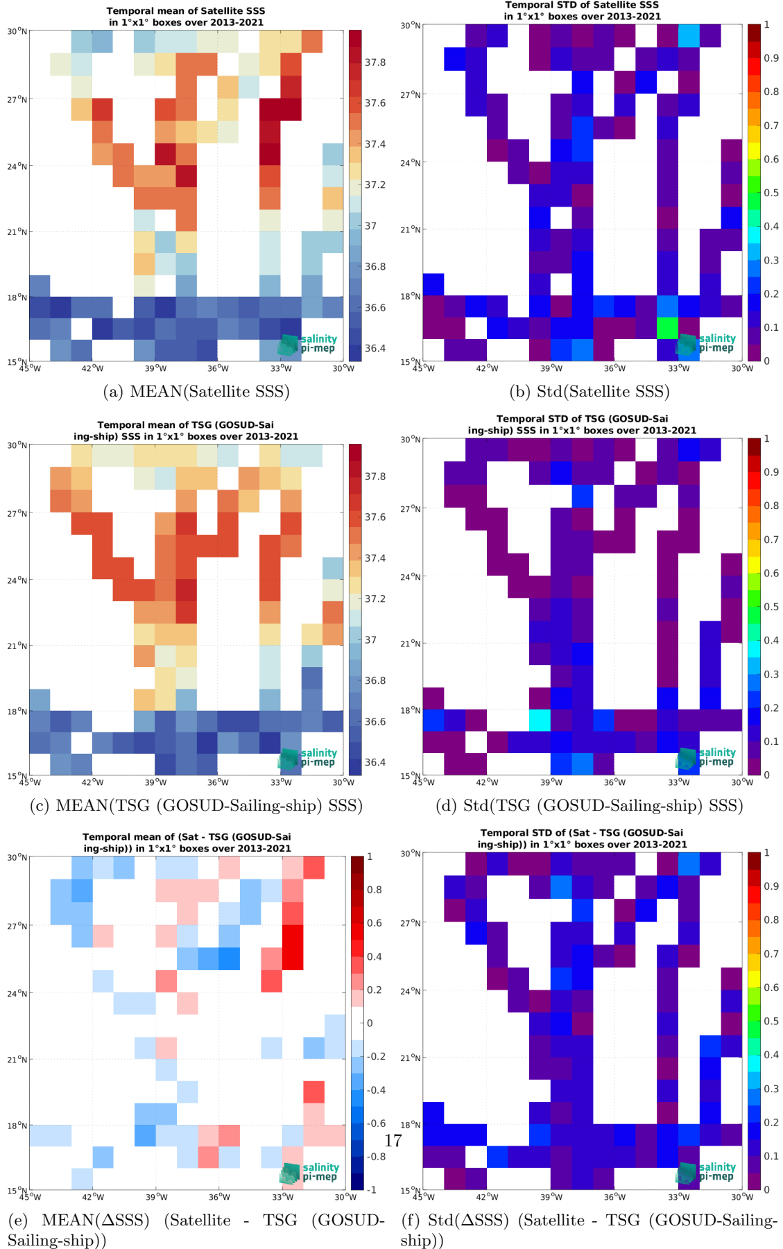
Figure 6: Temporal mean (left) and Std (right) of SSS from SMOS SSS L3 v9 - 9 Days (CATDS-CEC-LOCEAN) (top), TSG (GOSUD-Sailing-ship) (middle), and of \Delta SSS (Satellite - TSG (GOSUD-Sailing-ship)). Only match-up pairs are used to generate these maps.
