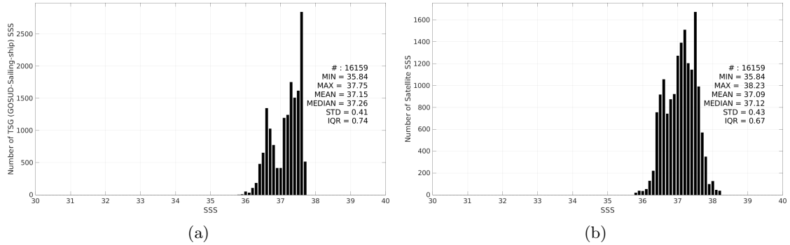
Figure 2: Histograms of SSS from TSG (GOSUD-Sailing-ship) (a) and SMOS SSS L3 v9 - 9 Days (CATDS-CEC-LOCEAN) (b) considering all match-up pairs per bins of 0.1 over the SPURS 1 Pi-MEP region and for the full satellite product period.
