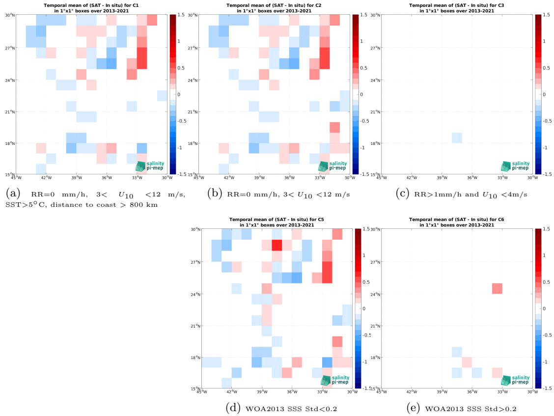
Figure 12: Temporal mean gridded over spatial boxes of size 1^{\circ} \times 1^{\circ} of \Delta\text{SSS} (SMOS SSS L3 v9 - 9 Days (CATDS-CEC-LOCEAN) - TSG (GOSUD-Sailing-ship)) for 5 different subdatasets corresponding to: RR=0 mm/h, 3 < U_{10} < 12 m/s, SST > 5^{\circ}\text{C} , distance to coast > 800 km (a), RR=0 mm/h, 3 < U_{10} < 12 m/s (b), RR > 1\text{mm/h} and U_{10} < 4\text{m/s} (c), WOA2013 SSS Std < 0.2 (d), WOA2013 SSS Std > 0.2 (e).
