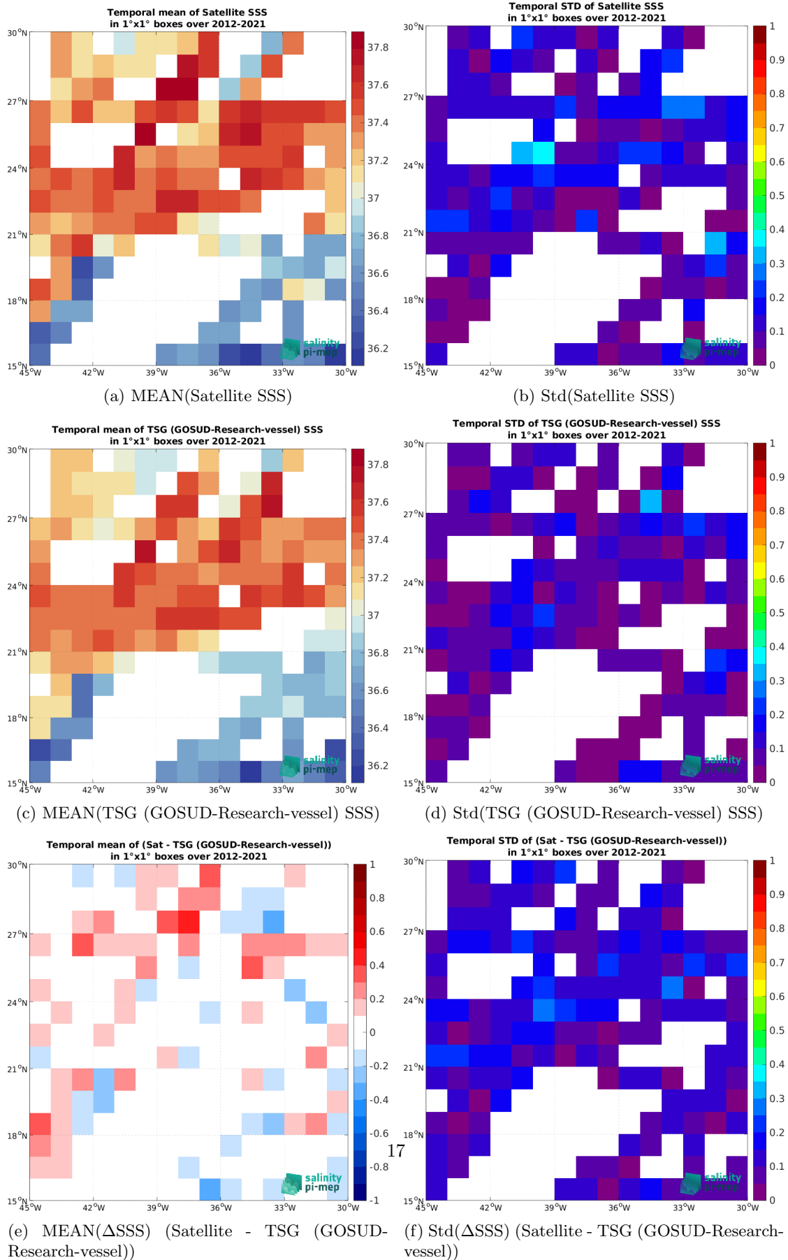
Figure 7: Temporal mean (left) and Std (right) of SSS from SMOS SSS L3 v9 - 9 Days (CATDS-CEC-LOCEAN) (top), TSG (GOSUD-Research-vessel) (middle), and of \Delta SSS (Satellite - TSG (GOSUD-Research-vessel)). Only match-up pairs are used to generate these maps.
