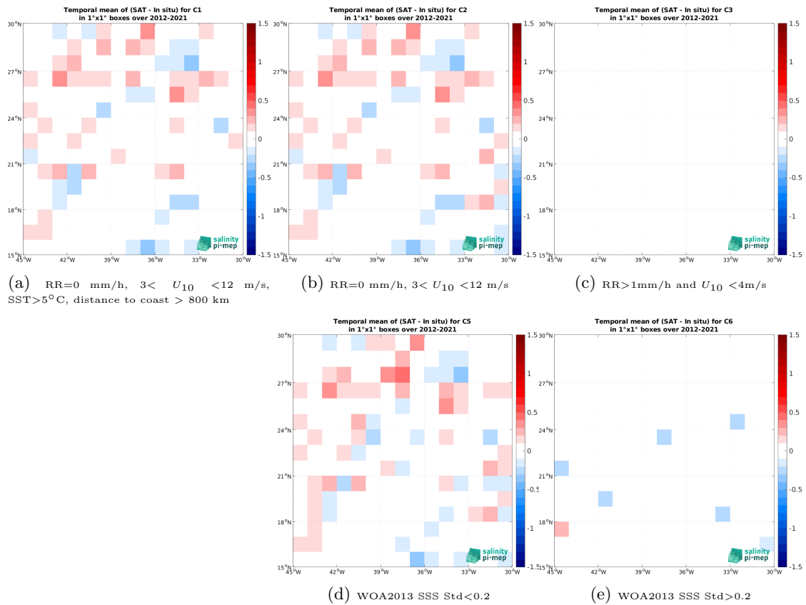
Figure 14: Temporal mean gridded over spatial boxes of size 1^\circ \times 1^\circ of \Delta SSS (SMOS SSS L3 v9 - 9 Days (CATDS-CEC-LOCEAN) - TSG (GOSUD-Research-vessel)) for 5 different subdatasets corresponding to: RR=0 mm/h, 3 < U_{10} < 12 m/s, SST > 5^\circ\text{C} , distance to coast > 800 km (a), RR=0 mm/h, 3 < U_{10} < 12 m/s (b), RR > 1 mm/h and U_{10} < 4 m/s (c), WOA2013 SSS Std < 0.2 (d), WOA2013 SSS Std > 0.2 (e).
