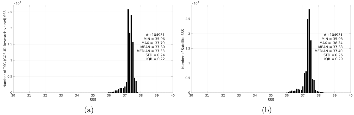
Figure 3: Histograms of SSS from TSG (GOSUD-Research-vessel) (a) and SMOS SSS L3 v9 - 9 Days (CATDS-CEC-LOCEAN) (b) considering all match-up pairs per bins of 0.1 over the SPURS 1 Pi-MEP region and for the full satellite product period.
