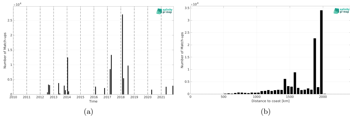
Figure 1: Number of match-ups between TSG (GOSUD-Research-vessel) and SMOS SSS L3 v9 - 9 Days (CATDS-CEC-LOCEAN) SSS as a function of time (a) and as function of the distance to coast (b) over the SPURS 1 Pi-MEP region and for the full satellite product period.
