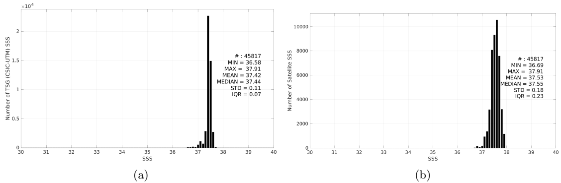
Figure 3: Histograms of SSS from TSG (CSIC-UTM) (a) and SMOS SSS L3 v9 - 9 Days (CATDS-CEC-LOCEAN) (b) considering all match-up pairs per bins of 0.1 over the SPURS 1 Pi-MEP region and for the full satellite product period.
