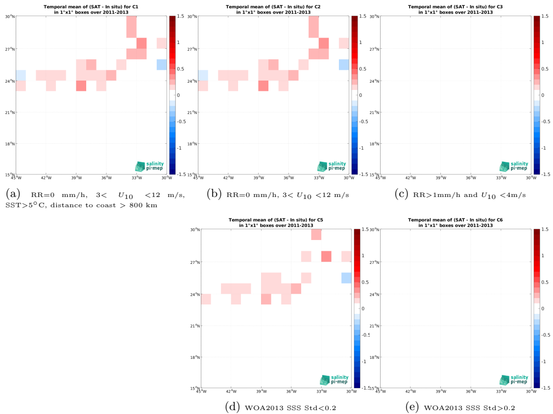
Figure 14: Temporal mean gridded over spatial boxes of size 1^\circ \times 1^\circ of \Delta SSS (SMOS SSS L3 v9 - 9 Days (CATDS-CEC-LOCEAN) - TSG (CSIC-UTM)) for 5 different subdatasets corresponding to:RR=0 mm/h, 3 < U_{10} < 12 m/s, SST >5^\circ C, distance to coast > 800 km (a), RR=0 mm/h, 3 < U_{10} < 12 m/s (b), RR >1 mm/h and U_{10} < 4 m/s (c), WOA2013 SSS Std <0.2 (d), WOA2013 SSS Std >0.2 (e).
