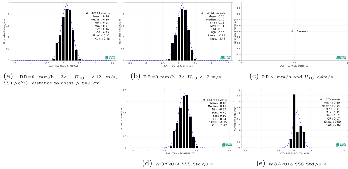
Figure 15: Normalized histogram of \Delta SSS (SMOS SSS L3 v9 - 9 Days (CATDS-CEC-LOCEAN) - TSG (CSIC-UTM)) for 5 different subdatasets corresponding to: RR=0 mm/h, 3 < U_{10} < 12 m/s, SST > 5°C, distance to coast > 800 km (a), RR=0 mm/h, 3 < U_{10} < 12 m/s (b), RR > 1mm/h and U_{10} < 4 m/s (c), WOA2013 SSS Std < 0.2 (d), WOA2013 SSS Std > 0.2 (e).
