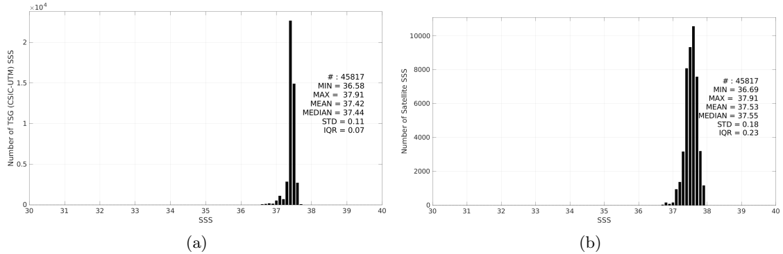
Figure 2: Histograms of SSS from TSG (CSIC-UTM) (a) and SMOS SSS L3 v9 - 9 Days (CATDS-CEC-LOCEAN) (b) considering all match-up pairs per bins of 0.1 over the SPURS 1 Pi-MEP region and for the full satellite product period.
