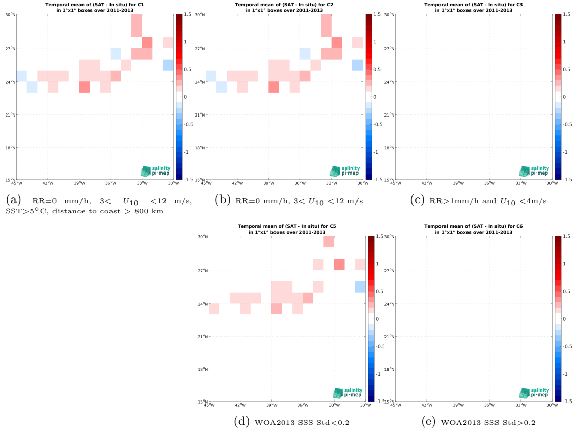
Figure 12: Temporal mean gridded over spatial boxes of size 1^{\circ}\times 1^{\circ} of \Delta\text{SSS} (SMOS SSS L3 v9 - 9 Days (CATDS-CEC-LOCEAN) - TSG (CSIC-UTM)) for 5 different subdatasets corresponding to:RR=0 mm/h, 3 < U_{10} < 12 m/s, SST >5^{\circ}\text{C} , distance to coast > 800 km (a), RR=0 mm/h, 3 < U_{10} < 12 m/s (b), RR >1 mm/h and U_{10} < 4 m/s (c), WOA2013 SSS Std <0.2 (d), WOA2013 SSS Std >0.2 (e).
