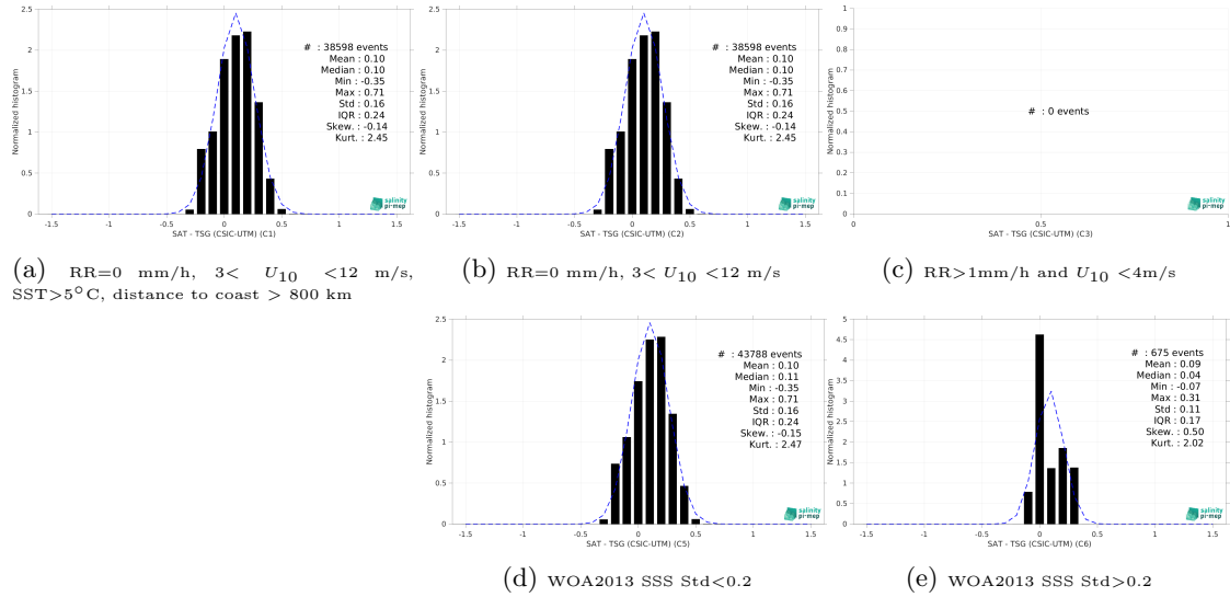
Figure 13: Normalized histogram of \Delta SSS (SMOS SSS L3 v9 - 9 Days (CATDS-CEC-LOCEAN) - TSG (CSIC-UTM)) for 5 different subdatasets corresponding to: RR=0 mm/h, 3 < U_{10} < 12 m/s, SST > 5°C, distance to coast > 800 km (a), RR=0 mm/h, 3 < U_{10} < 12 m/s (b), RR > 1mm/h and U_{10} < 4 m/s (c), WOA2013 SSS Std < 0.2 (d), WOA2013 SSS Std > 0.2 (e).
