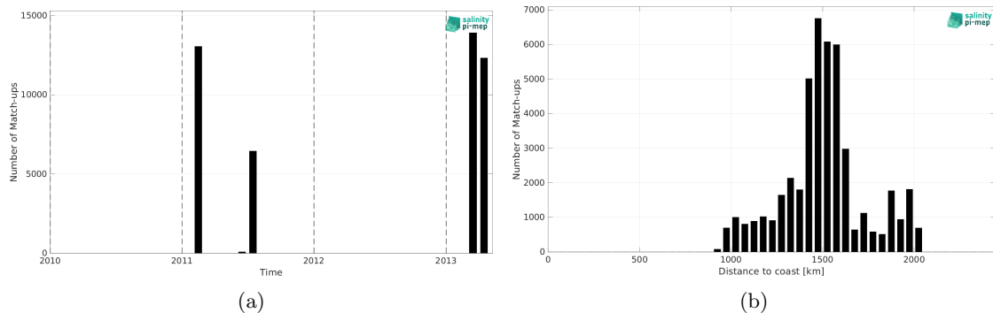
Figure 1: Number of match-ups between TSG (CSIC-UTM) and SMOS SSS L3 v9 - 9 Days (CATDS-CEC-LOCEAN) SSS as a function of time (a) and as function of the distance to coast (b) over the SPURS 1 Pi-MEP region and for the full satellite product period.
