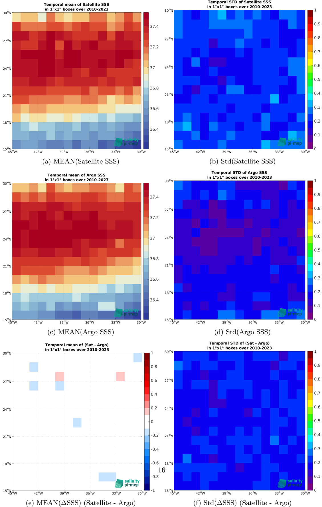
Figure 6: Temporal mean (left) and Std (right) of SSS from SMOS SSS L3 v9 - 9 Days (CATDS-CEC-LOCEAN) (top), Argo (middle), and of \Delta SSS (Satellite - Argo). Only match-up pairs are used to generate these maps.
