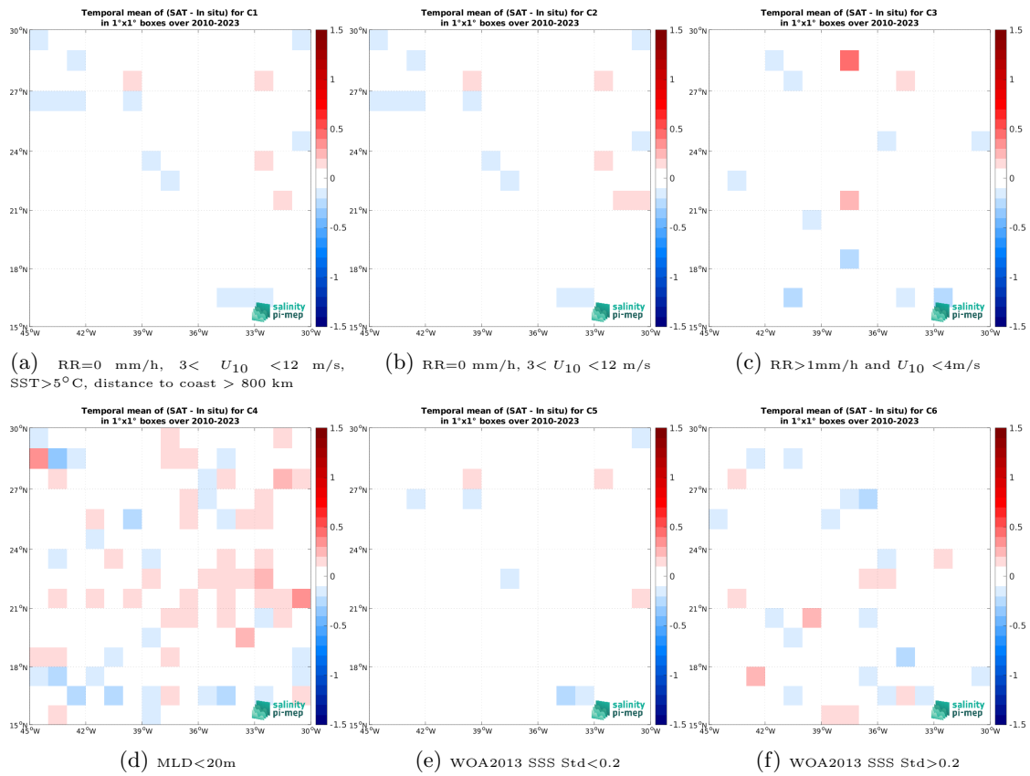
Figure 12: Temporal mean gridded over spatial boxes of size 1^\circ \times 1^\circ of \Delta SSS (SMOS SSS L3 v9 - 9 Days (CATDS-CEC-LOCEAN) - Argo) for 6 different subdatasets corresponding to:RR=0 mm/h, 3 < U_{10} < 12 m/s, SST >5^\circ\text{C} , distance to coast > 800 km (a), RR=0 mm/h, 3 < U_{10} < 12 m/s (b), RR >1 mm/h and U_{10} < 4 m/s (c),MLD <20 m (d),WOA2013 SSS Std <0.2 (e),WOA2013 SSS Std >0.2 (f).
