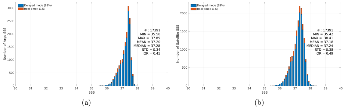
Figure 2: Histograms of SSS from Argo (a) and SMOS SSS L3 v9 - 9 Days (CATDS-CEC-LOCEAN) (b) considering all match-up pairs per bins of 0.1 over the SPURS 1 Pi-MEP region and for the full satellite product period.
