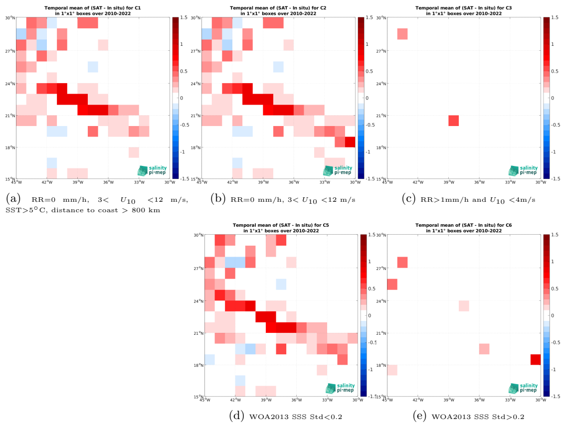
Figure 14: Temporal mean gridded over spatial boxes of size 1^\circ \times 1^\circ of \Delta SSS (SMOS SSS L3 v9 - 18 Days (CATDS-CEC-LOCEAN) - TSG (SAMOS)) for 5 different subdatasets corresponding to:RR=0 mm/h, 3 < U_{10} < 12 m/s, SST>5°C, distance to coast > 800 km (a), RR=0 mm/h, 3 < U_{10} < 12 m/s (b), RR>1mm/h and U_{10} < 4 m/s (c), WOA2013 SSS Std<0.2 (d), WOA2013 SSS Std>0.2 (e).
