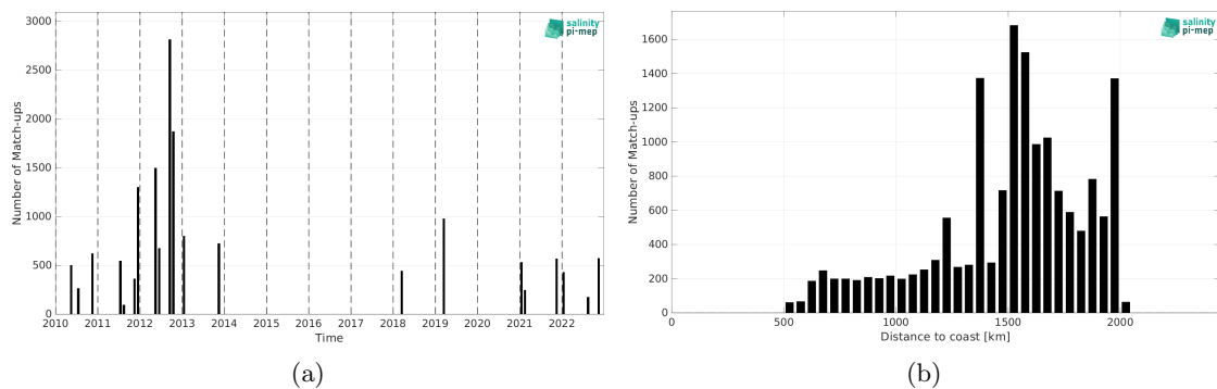
Figure 2: Number of match-ups between TSG (SAMOS) and SMOS SSS L3 v9 - 18 Days (CATDS-CEC-LOCEAN) SSS as a function of time (a) and as function of the distance to coast (b) over the SPURS 1 Pi-MEP region and for the full satellite product period.
