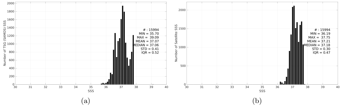
Figure 3: Histograms of SSS from TSG (SAMOS) (a) and SMOS SSS L3 v9 - 18 Days (CATDS-CEC-LOCEAN) (b) considering all match-up pairs per bins of 0.1 over the SPURS 1 Pi-MEP region and for the full satellite product period.
