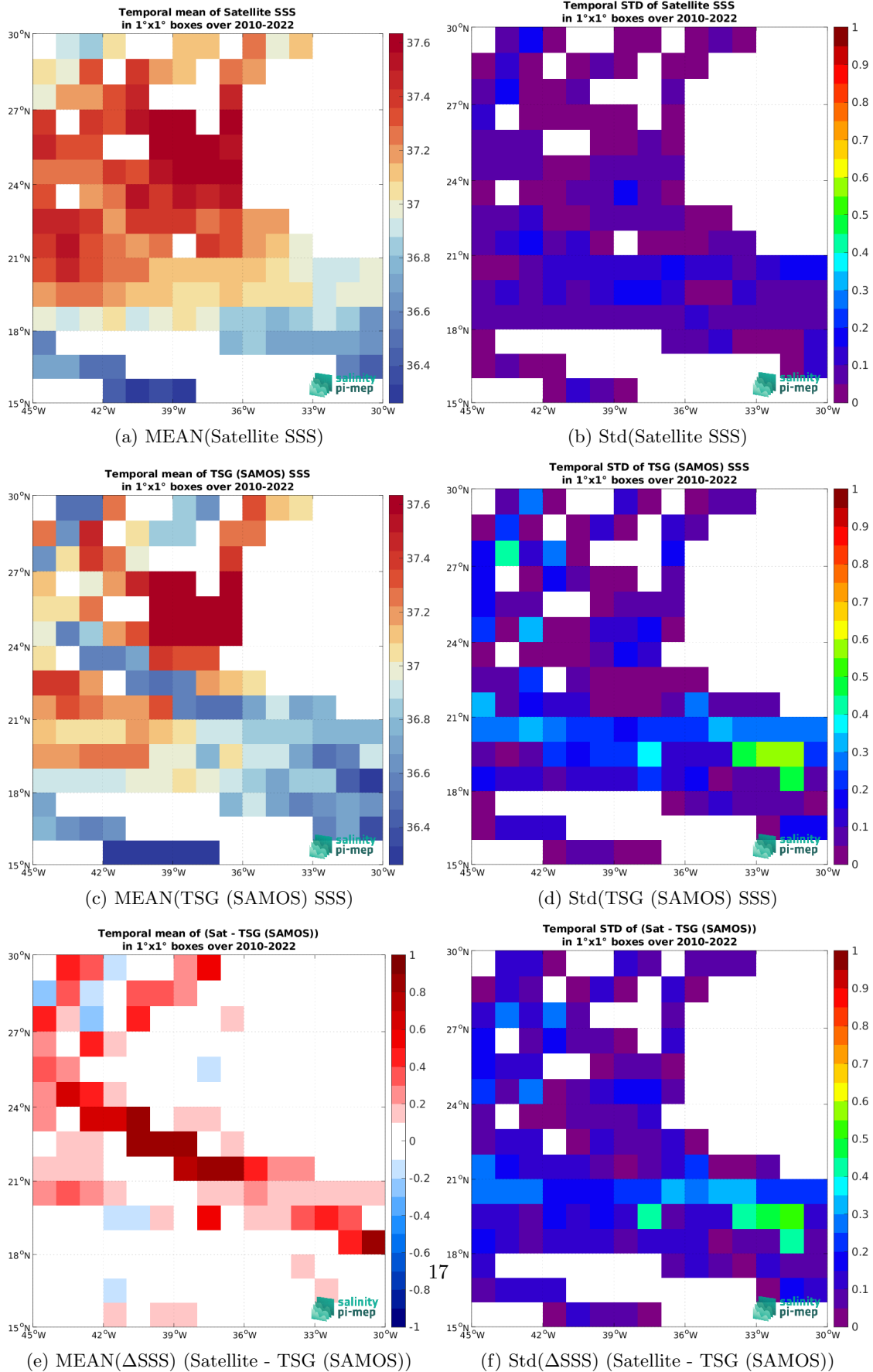
Figure 6: Temporal mean (left) and Std (right) of SSS from SMOS SSS L3 v9 - 18 Days (CATDS-CEC-LOCEAN) (top), TSG (SAMOS) (middle), and of \Delta SSS (Satellite - TSG (SAMOS)). Only match-up pairs are used to generate these maps.
