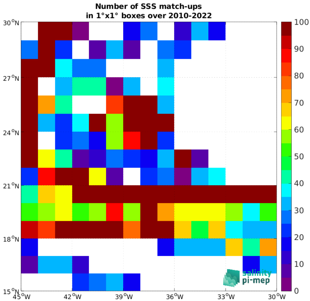
Figure 4: Number of SSS match-ups between TSG (SAMOS) SSS and the SMOS SSS L3 v9 - 18 Days (CATDS-CEC-LOCEAN) SSS product for the SPURS 1 Pi-MEP region over 1°x1° boxes and for the full satellite product period.
