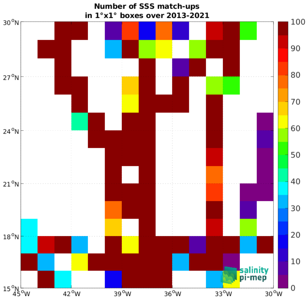
Figure 5: Number of SSS match-ups between TSG (GOSUD-Sailing-ship) SSS and the SMOS SSS L3 v9 - 18 Days (CATDS-CEC-LOCEAN) SSS product for the SPURS 1 Pi-MEP region over 1^\circ \times 1^\circ boxes and for the full satellite product period.
