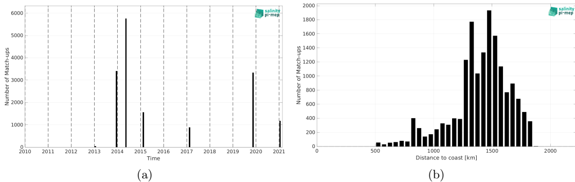
Figure 2: Number of match-ups between TSG (GOSUD-Sailing-ship) and SMOS SSS L3 v9 - 18 Days (CATDS-CEC-LOCEAN) SSS as a function of time (a) and as function of the distance to coast (b) over the SPURS 1 Pi-MEP region and for the full satellite product period.
