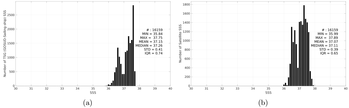
Figure 3: Histograms of SSS from TSG (GOSUD-Sailing-ship) (a) and SMOS SSS L3 v9 - 18 Days (CATDS-CEC-LOCEAN) (b) considering all match-up pairs per bins of 0.1 over the SPURS 1 Pi-MEP region and for the full satellite product period.
