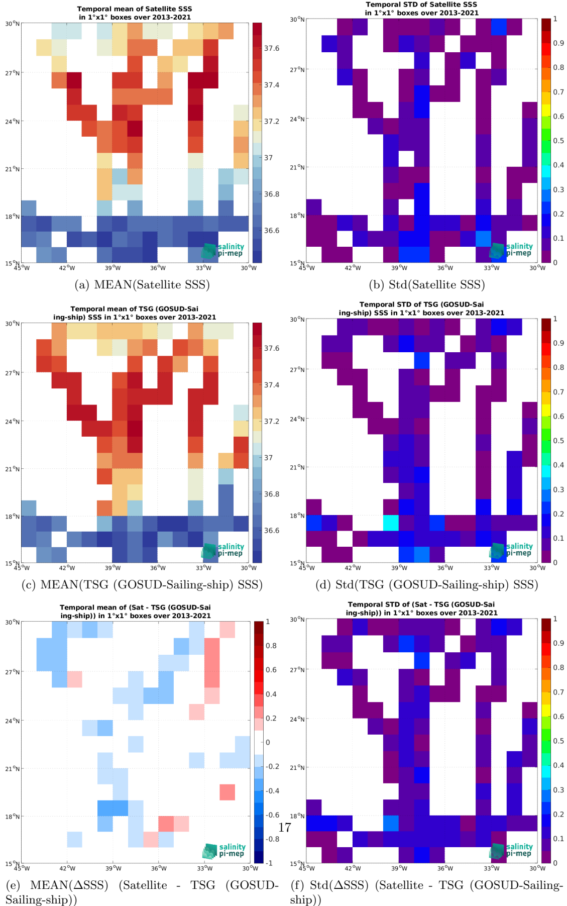
Figure 7: Temporal mean (left) and Std (right) of SSS from SMOS SSS L3 v9 - 18 Days (CATDS-CEC-LOCEAN) (top), TSG (GOSUD-Sailing-ship) (middle), and of \Delta SSS (Satellite - TSG (GOSUD-Sailing-ship)). Only match-up pairs are used to generate these maps.
