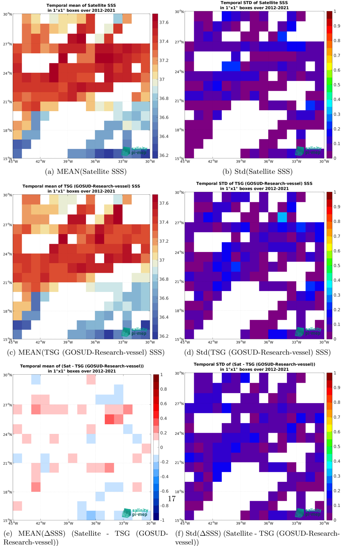
Figure 7: Temporal mean (left) and Std (right) of SSS from SMOS SSS L3 v9 - 18 Days (CATDS-CEC-LOCEAN) (top), TSG (GOSUD-Research-vessel) (middle), and of \Delta SSS (Satellite - TSG (GOSUD-Research-vessel)). Only match-up pairs are used to generate these maps.
