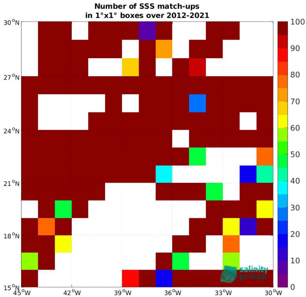
Figure 5: Number of SSS match-ups between TSG (GOSUD-Research-vessel) SSS and the SMOS SSS L3 v9 - 18 Days (CATDS-CEC-LOCEAN) SSS product for the SPURS 1 Pi-MEP region over 1^\circ \times 1^\circ boxes and for the full satellite product period.
