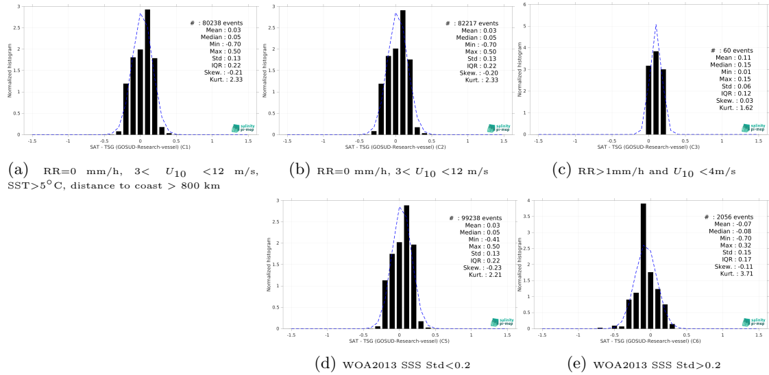
Figure 15: Normalized histogram of \Delta\text{SSS} (SMOS SSS L3 v9 - 18 Days (CATDS-CEC-LOCEAN) - TSG (GOSUD-Research-vessel)) for 5 different subdatasets corresponding to: RR=0 mm/h, 3 < U_{10} < 12 m/s, SST > 5^{\circ}\text{C} , distance to coast > 800 km (a), RR=0 mm/h, 3 < U_{10} < 12 m/s (b), RR > 1\text{mm/h} and U_{10} < 4\text{m/s} (c), WOA2013 SSS \text{Std} < 0.2 (d), WOA2013 SSS \text{Std} > 0.2 (e).
