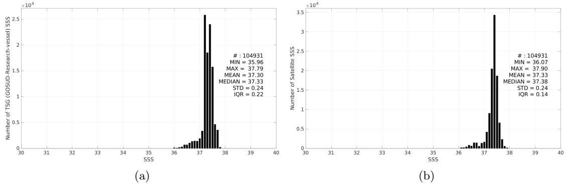
Figure 3: Histograms of SSS from TSG (GOSUD-Research-vessel) (a) and SMOS SSS L3 v9 - 18 Days (CATDS-CEC-LOCEAN) (b) considering all match-up pairs per bins of 0.1 over the SPURS 1 Pi-MEP region and for the full satellite product period.
