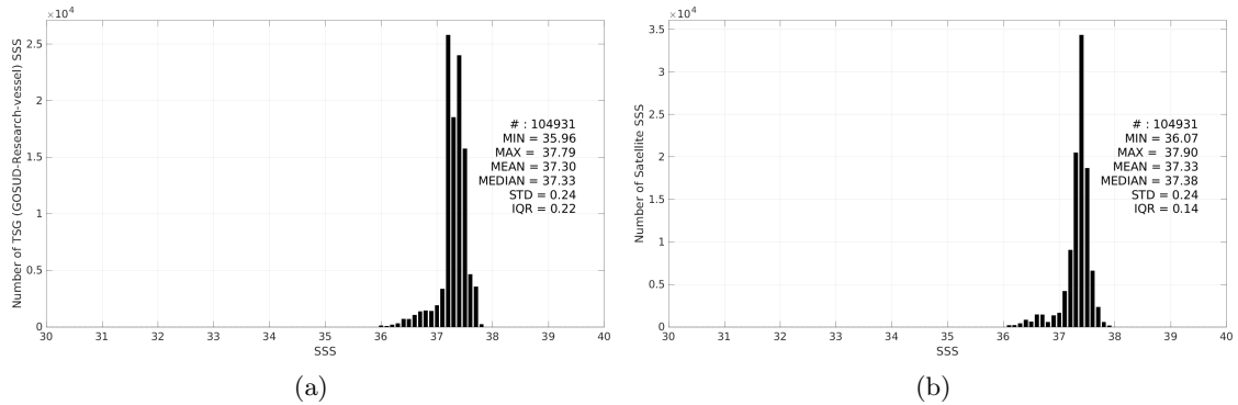
Figure 2: Histograms of SSS from TSG (GOSUD-Research-vessel) (a) and SMOS SSS L3 v9 - 18 Days (CATDS-CEC-LOCEAN) (b) considering all match-up pairs per bins of 0.1 over the SPURS 1 Pi-MEP region and for the full satellite product period.
