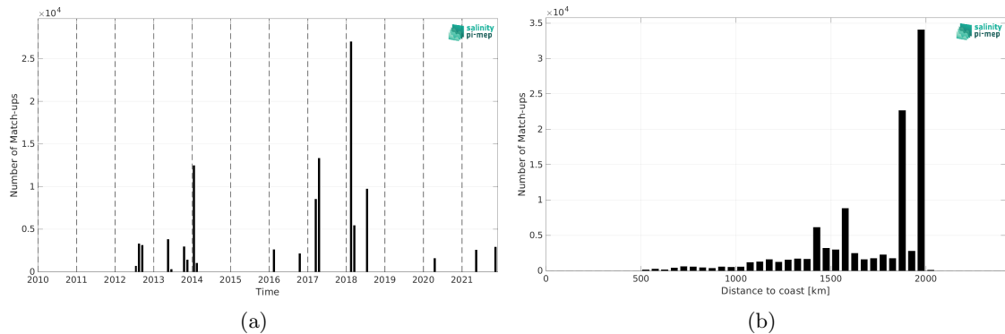
Figure 1: Number of match-ups between TSG (GOSUD-Research-vessel) and SMOS SSS L3 v9 - 18 Days (CATDS-CEC-LOCEAN) SSS as a function of time (a) and as function of the distance to coast (b) over the SPURS 1 Pi-MEP region and for the full satellite product period.
