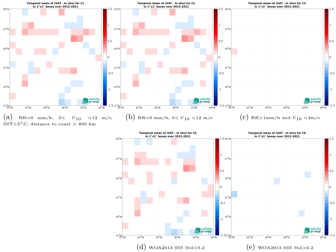
Figure 12: Temporal mean gridded over spatial boxes of size 1^\circ \times 1^\circ of \Delta\text{SSS} (SMOS SSS L3 v9 - 18 Days (CATDS-CEC-LOCEAN) - TSG (GOSUD-Research-vessel)) for 5 different subdatasets corresponding to: RR=0 mm/h, 3 < U_{10} < 12 m/s, SST > 5^\circ\text{C} , distance to coast > 800 km (a), RR=0 mm/h, 3 < U_{10} < 12 m/s (b), RR > 1\text{mm/h} and U_{10} < 4\text{m/s} (c), WOA2013 SSS Std < 0.2 (d), WOA2013 SSS Std > 0.2 (e).
