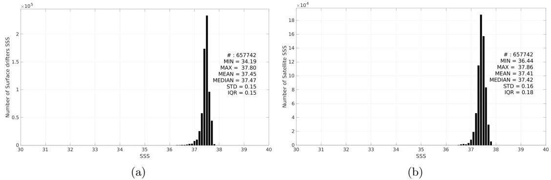
Figure 2: Histograms of SSS from Surface drifters (a) and SMOS SSS L3 v9 - 18 Days (CATDS-CEC-LOCEAN) (b) considering all match-up pairs per bins of 0.1 over the SPURS 1 Pi-MEP region and for the full satellite product period.
