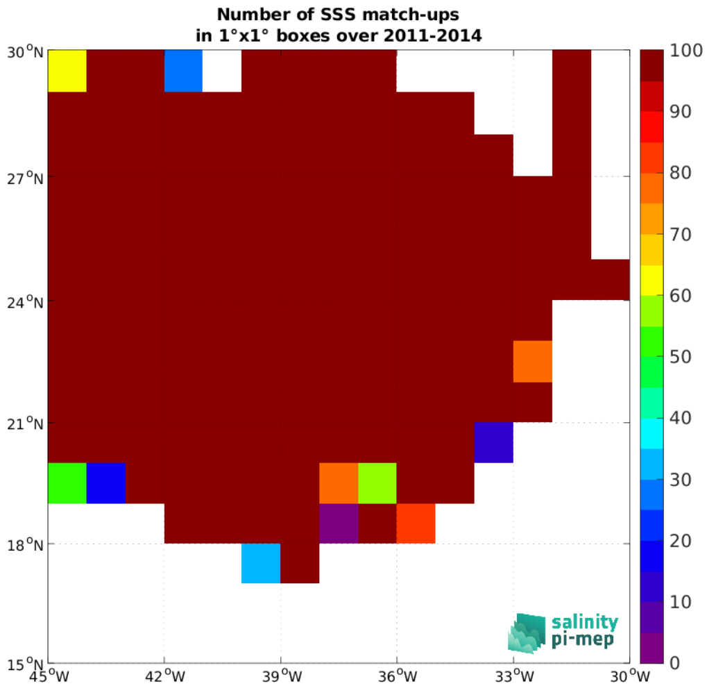
Figure 3: Number of SSS match-ups between Surface drifters SSS and the SMOS SSS L3 v9 - 18 Days (CATDS-CEC-LOCEAN) SSS product for the SPURS 1 Pi-MEP region over 1°x1° boxes and for the full satellite product period.
