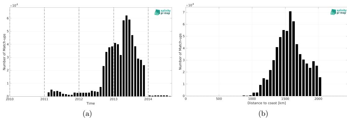
Figure 1: Number of match-ups between Surface drifters and SMOS SSS L3 v9 - 18 Days (CATDS-CEC-LOCEAN) SSS as a function of time (a) and as function of the distance to coast (b) over the SPURS 1 Pi-MEP region and for the full satellite product period.
