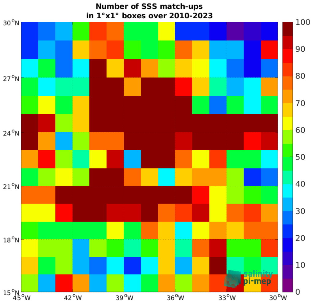
Figure 5: Number of SSS match-ups between Argo SSS and the SMOS SSS L3 v9 - 18 Days (CATDS-CEC-LOCEAN) SSS product for the SPURS 1 Pi-MEP region over 1^\circ \times 1^\circ boxes and for the full satellite product period.
