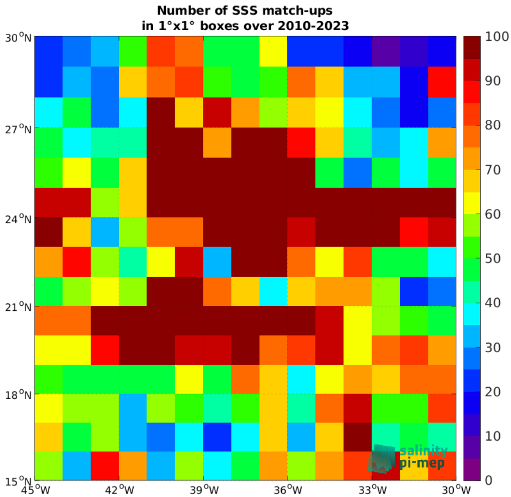
Figure 5: Number of SSS match-ups between Argo SSS and the SMOS SSS L3 v9 - 18 Days (CATDS-CEC-LOCEAN) SSS product for the SPURS 1 Pi-MEP region over 1°x1° boxes and for the full satellite product period.
