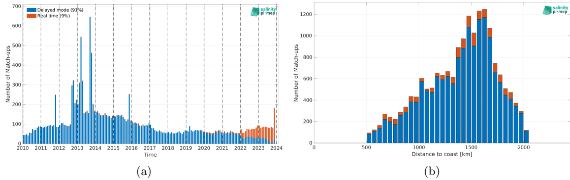
Figure 2: Number of match-ups between Argo and SMOS SSS L3 v9 - 18 Days (CATDS-CEC-LOCEAN) SSS as a function of time (a) and as function of the distance to coast (b) over the SPURS 1 Pi-MEP region and for the full satellite product period.
