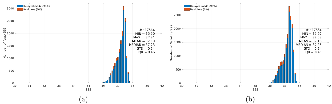
Figure 3: Histograms of SSS from Argo (a) and SMOS SSS L3 v9 - 18 Days (CATDS-CEC-LOCEAN) (b) considering all match-up pairs per bins of 0.1 over the SPURS 1 Pi-MEP region and for the full satellite product period.
