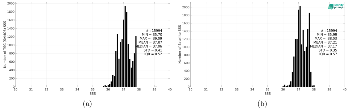
Figure 2: Histograms of SSS from TSG (SAMOS) (a) and SMOS SSS L3 v8 - 9 Days (CATDS-CEC-LOCEAN) (b) considering all match-up pairs per bins of 0.1 over the SPURS 1 Pi-MEP region and for the full satellite product period.
