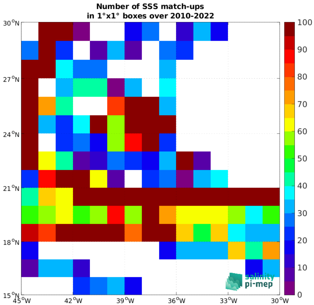
Figure 4: Number of SSS match-ups between TSG (SAMOS) SSS and the SMOS SSS L3 v8 - 9 Days (CATDS-CEC-LOCEAN) SSS product for the SPURS 1 Pi-MEP region over 1°x1° boxes and for the full satellite product period.
