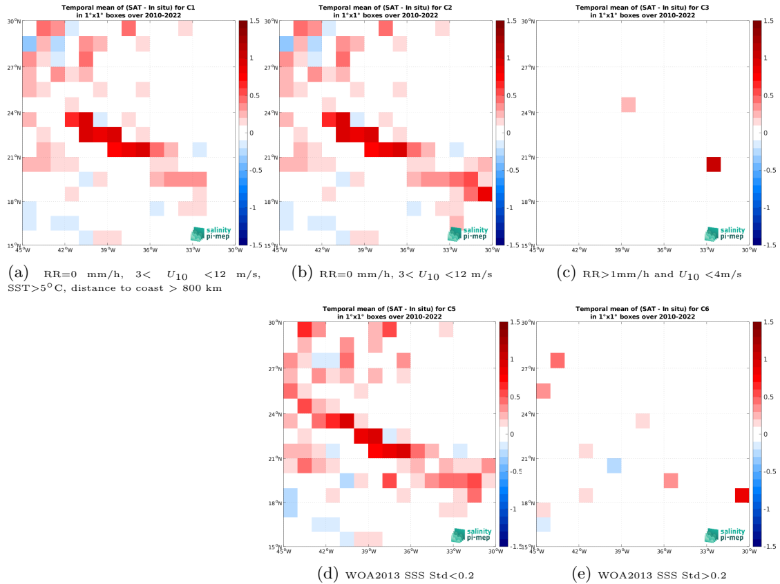
Figure 12: Temporal mean gridded over spatial boxes of size 1^{\circ}\times 1^{\circ} of \Delta\text{SSS} (SMOS SSS L3 v8 - 9 Days (CATDS-CEC-LOCEAN) - TSG (SAMOS)) for 5 different subdatasets corresponding to:RR=0 mm/h, 3 < U_{10} < 12 m/s, SST >5^{\circ}\text{C} , distance to coast > 800 km (a), RR=0 mm/h, 3 < U_{10} < 12 m/s (b), RR >1 mm/h and U_{10} < 4 m/s (c), WOA2013 SSS Std <0.2 (d), WOA2013 SSS Std >0.2 (e).
