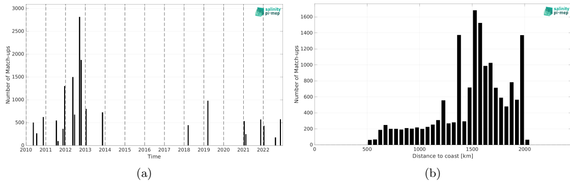
Figure 1: Number of match-ups between TSG (SAMOS) and SMOS SSS L3 v8 - 9 Days (CATDS-CEC-LOCEAN) SSS as a function of time (a) and as function of the distance to coast (b) over the SPURS 1 Pi-MEP region and for the full satellite product period.
