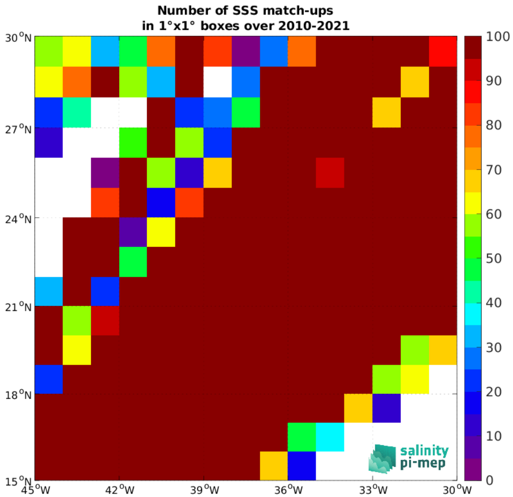
Figure 4: Number of SSS match-ups between TSG (LEGOS-DM) SSS and the SMOS SSS L3 v8 - 9 Days (CATDS-CEC-LOCEAN) SSS product for the SPURS 1 Pi-MEP region over 1°x1° boxes and for the full satellite product period.
