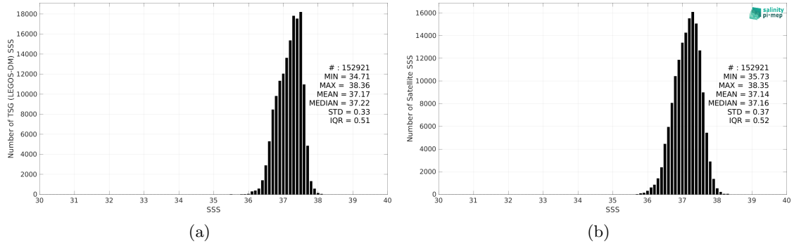
Figure 2: Histograms of SSS from TSG (LEGOS-DM) (a) and SMOS SSS L3 v8 - 9 Days (CATDS-CEC-LOCEAN) (b) considering all match-up pairs per bins of 0.1 over the SPURS 1 Pi-MEP region and for the full satellite product period.
