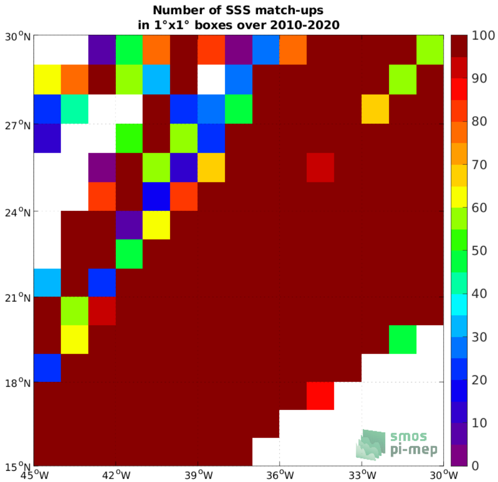
Figure 4: Number of SSS match-ups between TSG (LEGOS-DM) SSS and the SMOS SSS L3 v8 - 9 Days (CATDS-CECOS-LOCEAN) SSS product for the SPURS 1 Pi-MEP region over 1°x1° boxes and for the full satellite product period.
