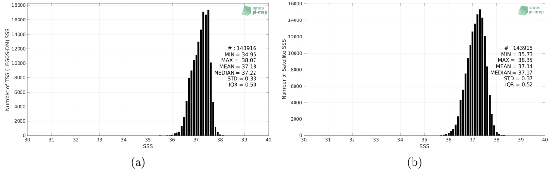
Figure 2: Histograms of SSS from TSG (LEGOS-DM) (a) and SMOS SSS L3 v8 - 9 Days (CATDS-CECOS-LOCEAN) (b) considering all match-up pairs per bins of 0.1 over the SPURS 1 Pi-MEP region and for the full satellite product period.
