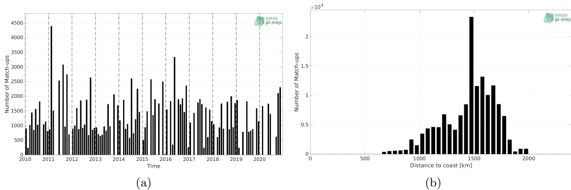
Figure 1: Number of match-ups between TSG (LEGOS-DM) and SMOS SSS L3 v8 - 9 Days (CATDS-CECOS-LOCEAN) SSS as a function of time (a) and as function of the distance to coast (b) over the SPURS 1 Pi-MEP region and for the full satellite product period.
