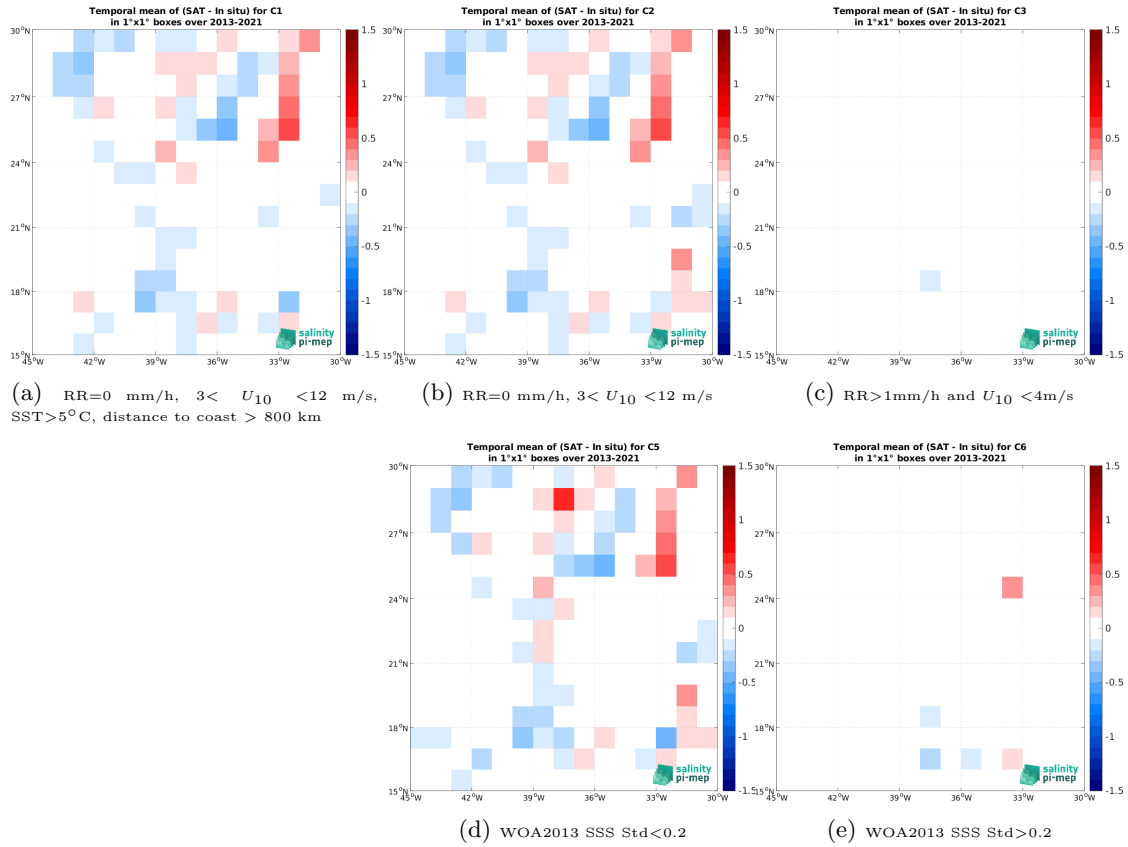
Figure 12: Temporal mean gridded over spatial boxes of size 1^{\circ} \times 1^{\circ} of \Delta\text{SSS} (SMOS SSS L3 v8 - 9 Days (CATDS-CEC-LOCEAN) - TSG (GOSUD-Sailing-ship)) for 5 different subdatasets corresponding to: RR=0 mm/h, 3 < U_{10} < 12 m/s, SST > 5^{\circ}\text{C} , distance to coast > 800 km (a), RR=0 mm/h, 3 < U_{10} < 12 m/s (b), RR > 1\text{mm/h} and U_{10} < 4\text{m/s} (c), WOA2013 SSS Std < 0.2 (d), WOA2013 SSS Std > 0.2 (e).
