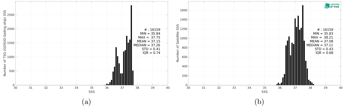
Figure 2: Histograms of SSS from TSG (GOSUD-Sailing-ship) (a) and SMOS SSS L3 v8 - 9 Days (CATDS-CEC-LOCEAN) (b) considering all match-up pairs per bins of 0.1 over the SPURS 1 Pi-MEP region and for the full satellite product period.
