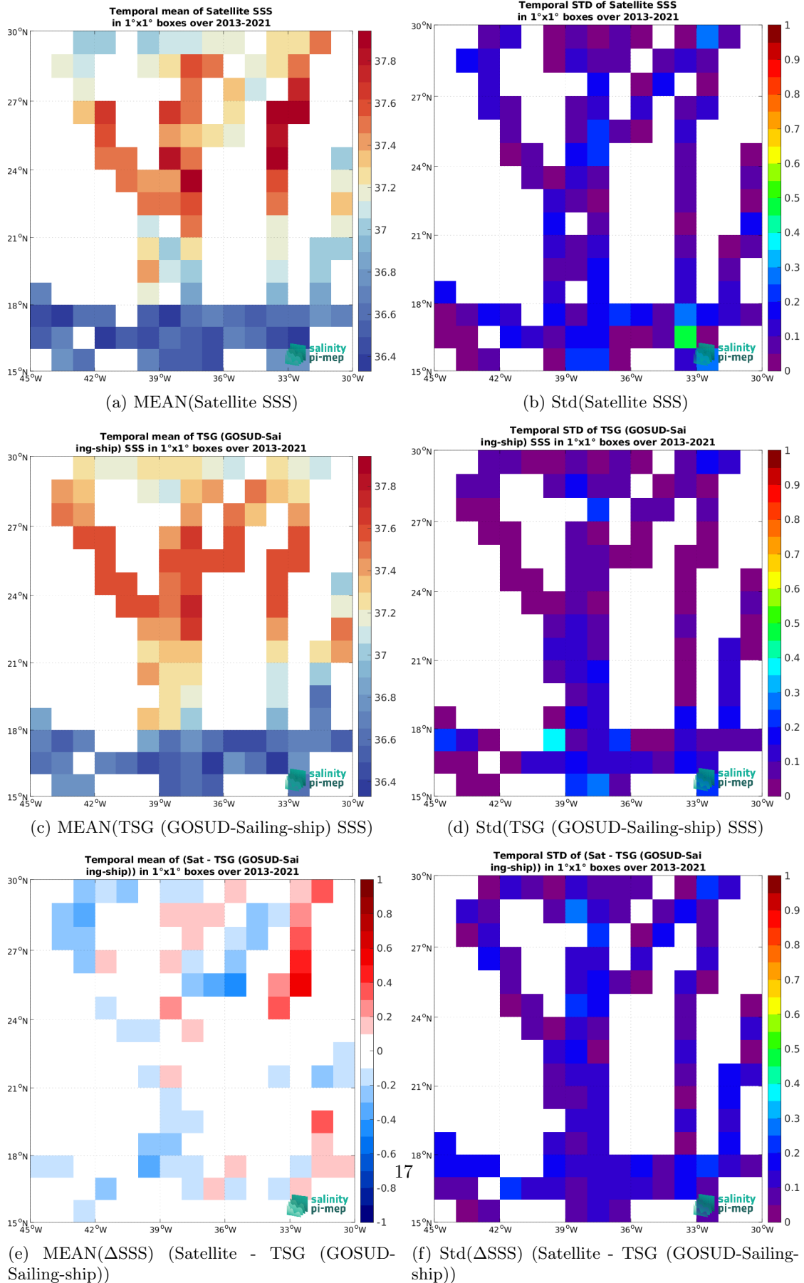
Figure 6: Temporal mean (left) and Std (right) of SSS from SMOS SSS L3 v8 - 9 Days (CATDS-CEC-LOCEAN) (top), TSG (GOSUD-Sailing-ship) (middle), and of \Delta SSS (Satellite - TSG (GOSUD-Sailing-ship)). Only match-up pairs are used to generate these maps.
