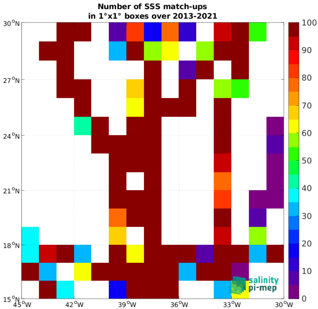
Figure 4: Number of SSS match-ups between TSG (GOSUD-Sailing-ship) SSS and the SMOS SSS L3 v8 - 9 Days (CATDS-CEC-LOCEAN) SSS product for the SPURS 1 Pi-MEP region over 1^\circ \times 1^\circ boxes and for the full satellite product period.
