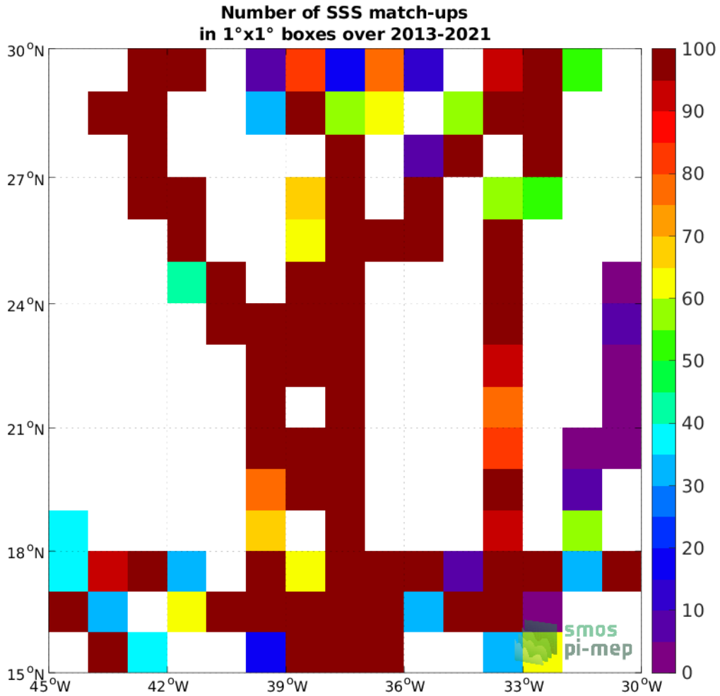
Figure 4: Number of SSS match-ups between TSG (GOSUD-Sailing-ship) SSS and the SMOS SSS L3 v8 - 9 Days (CATDS-CECOS-LOCEAN) SSS product for the SPURS 1 Pi-MEP region over 1°x1° boxes and for the full satellite product period.
