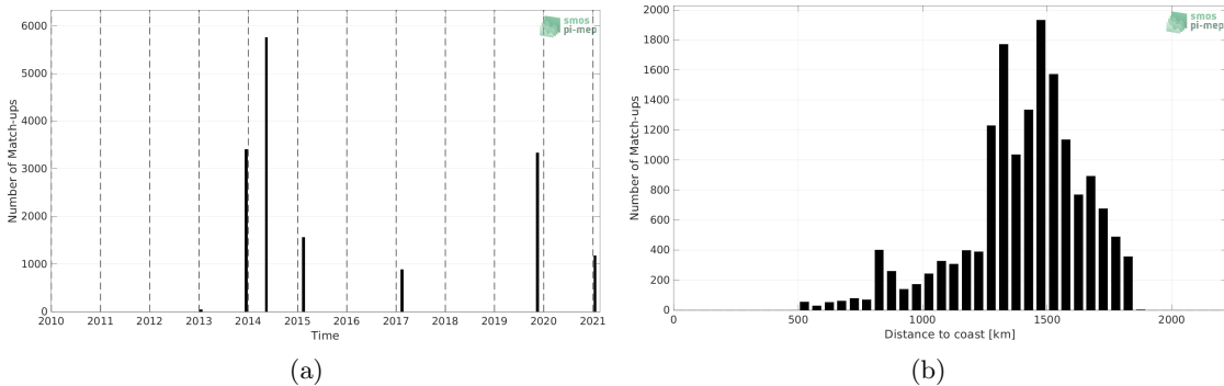
Figure 1: Number of match-ups between TSG (GOSUD-Sailing-ship) and SMOS SSS L3 v8 - 9 Days (CATDS-CECOS-LOCEAN) SSS as a function of time (a) and as function of the distance to coast (b) over the SPURS 1 Pi-MEP region and for the full satellite product period.
