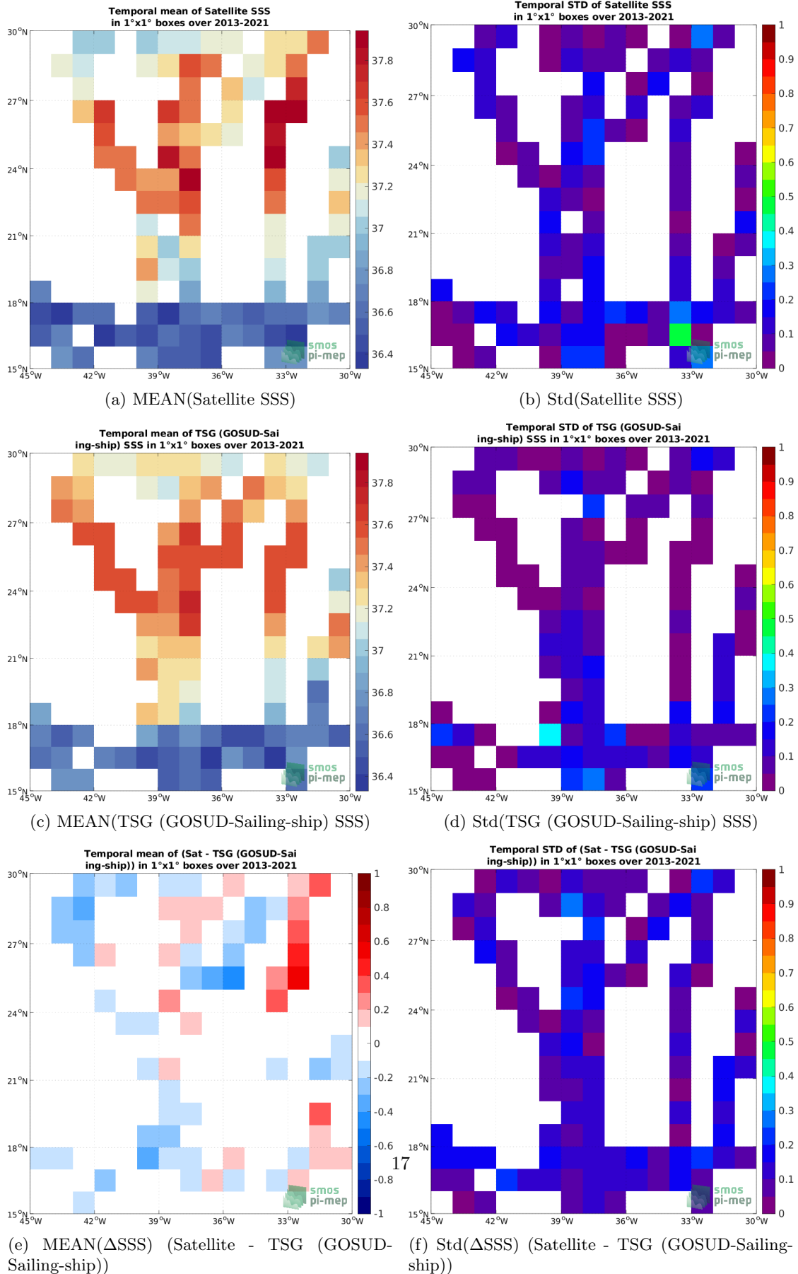
Figure 6: Temporal mean (left) and Std (right) of SSS from SMOS SSS L3 v8 - 9 Days (CATDS-CECOS-LOCEAN) (top), TSG (GOSUD-Sailing-ship) (middle), and of \Delta SSS (Satellite - TSG (GOSUD-Sailing-ship)). Only match-up pairs are used to generate these maps.
