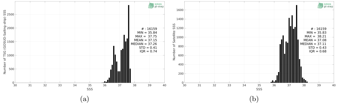
Figure 2: Histograms of SSS from TSG (GOSUD-Sailing-ship) (a) and SMOS SSS L3 v8 - 9 Days (CATDS-CECOS-LOCEAN) (b) considering all match-up pairs per bins of 0.1 over the SPURS 1 Pi-MEP region and for the full satellite product period.
