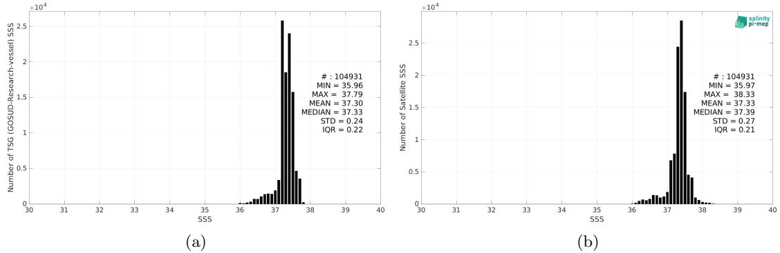
Figure 2: Histograms of SSS from TSG (GOSUD-Research-vessel) (a) and SMOS SSS L3 v8 - 9 Days (CATDS-CEC-LOCEAN) (b) considering all match-up pairs per bins of 0.1 over the SPURS 1 Pi-MEP region and for the full satellite product period.
