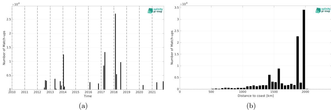
Figure 1: Number of match-ups between TSG (GOSUD-Research-vessel) and SMOS SSS L3 v8 - 9 Days (CATDS-CEC-LOCEAN) SSS as a function of time (a) and as function of the distance to coast (b) over the SPURS 1 Pi-MEP region and for the full satellite product period.
