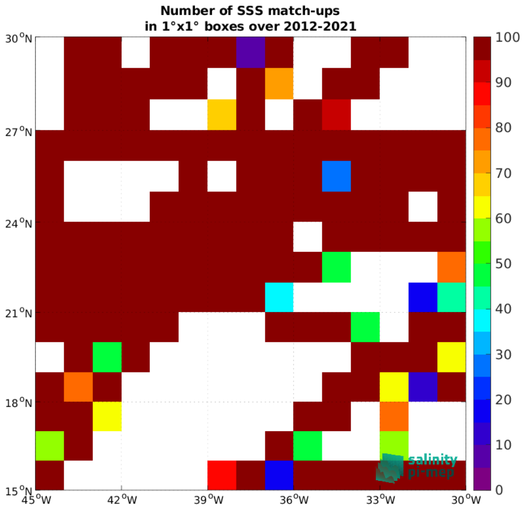
Figure 4: Number of SSS match-ups between TSG (GOSUD-Research-vessel) SSS and the SMOS SSS L3 v8 - 9 Days (CATDS-CEC-LOCEAN) SSS product for the SPURS 1 Pi-MEP region over 1^\circ \times 1^\circ boxes and for the full satellite product period.
