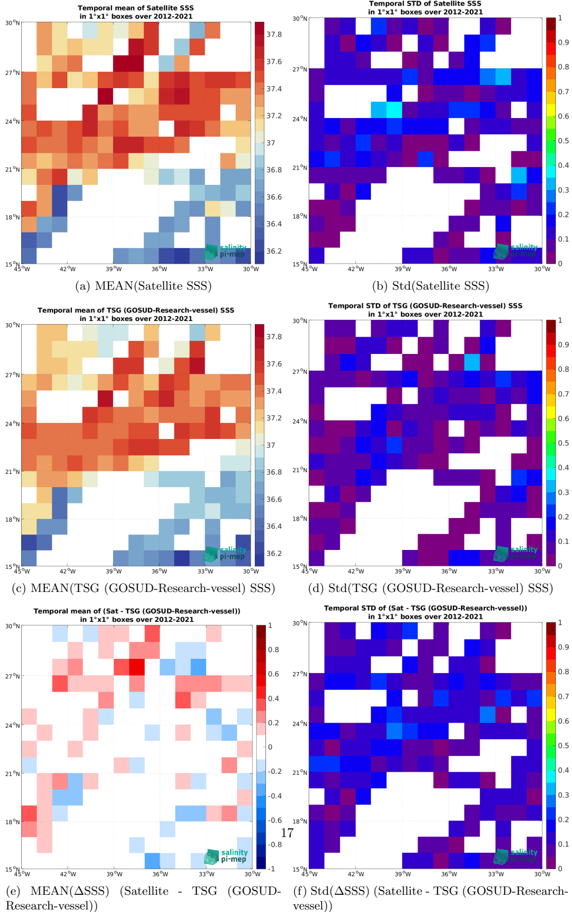
Figure 6: Temporal mean (left) and Std (right) of SSS from SMOS SSS L3 v8 - 9 Days (CATDS-CEC-LOCEAN) (top), TSG (GOSUD-Research-vessel) (middle), and of \Delta SSS (Satellite - TSG (GOSUD-Research-vessel)). Only match-up pairs are used to generate these maps.
