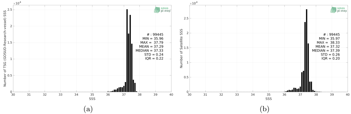
Figure 2: Histograms of SSS from TSG (GOSUD-Research-vessel) (a) and SMOS SSS L3 v8 - 9 Days (CATDS-CECOS-LOCEAN) (b) considering all match-up pairs per bins of 0.1 over the SPURS 1 Pi-MEP region and for the full satellite product period.
