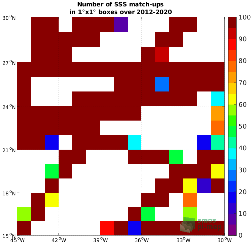
Figure 4: Number of SSS match-ups between TSG (GOSUD-Research-vessel) SSS and the SMOS SSS L3 v8 - 9 Days (CATDS-CECOS-LOCEAN) SSS product for the SPURS 1 Pi-MEP region over 1°x1° boxes and for the full satellite product period.
