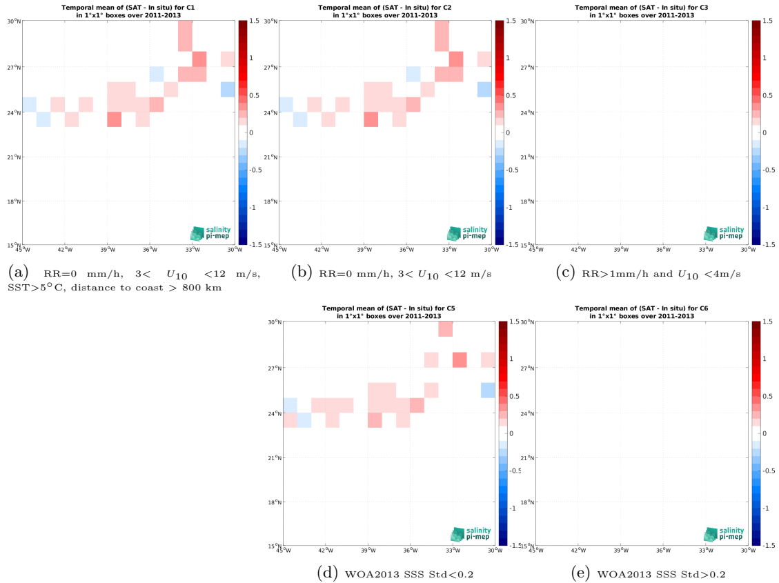
Figure 12: Temporal mean gridded over spatial boxes of size 1^{\circ}\times 1^{\circ} of \Delta\text{SSS} (SMOS SSS L3 v8 - 9 Days (CATDS-CEC-LOCEAN) - TSG (CSIC-UTM)) for 5 different subdatasets corresponding to:RR=0 mm/h, 3 < U_{10} < 12 m/s, SST >5^{\circ}\text{C} , distance to coast > 800 km (a), RR=0 mm/h, 3 < U_{10} < 12 m/s (b), RR >1 mm/h and U_{10} < 4 m/s (c), WOA2013 SSS Std <0.2 (d), WOA2013 SSS Std >0.2 (e).
