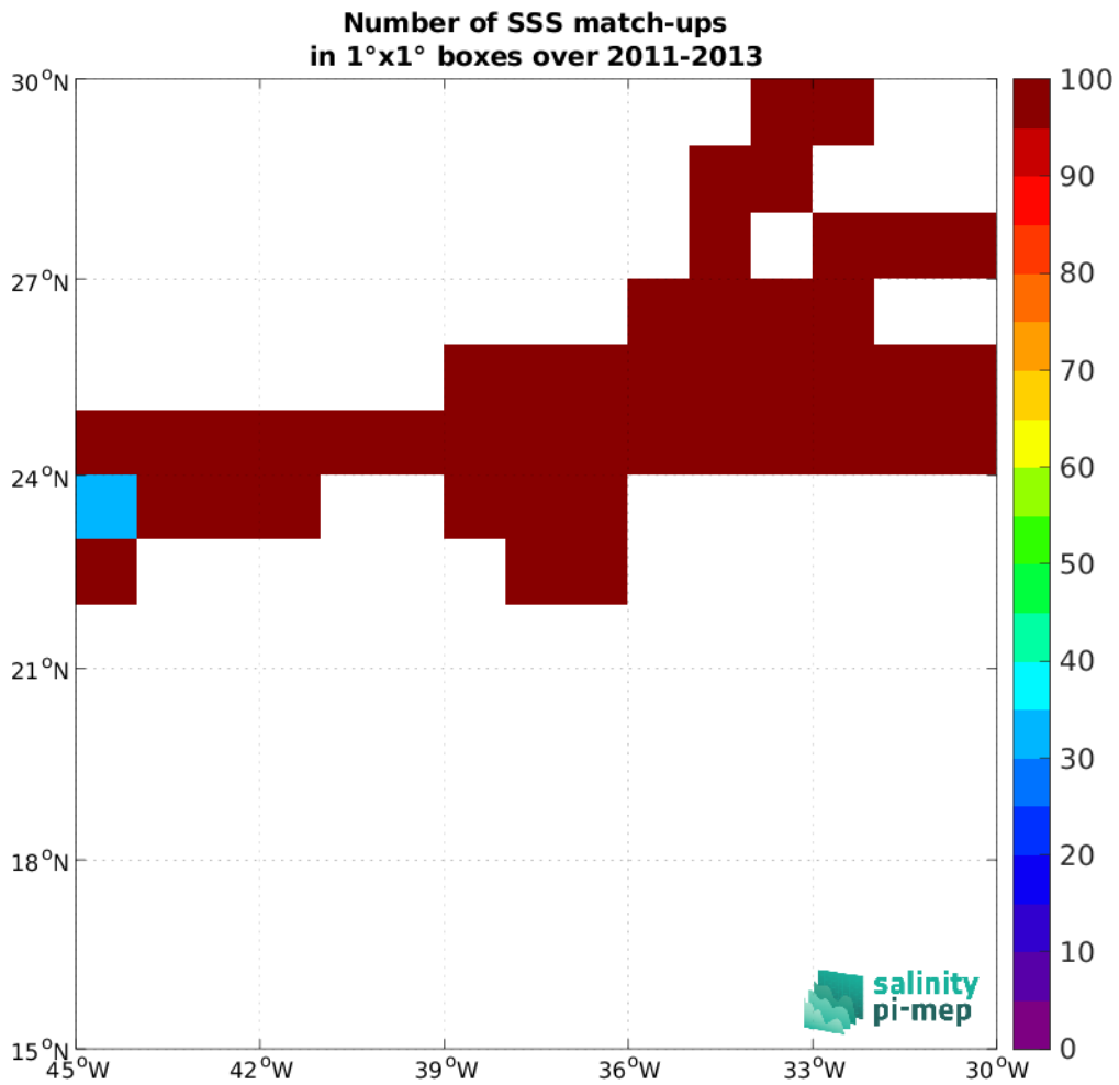
Figure 4: Number of SSS match-ups between TSG (CSIC-UTM) SSS and the SMOS SSS L3 v8 - 9 Days (CATDS-CEC-LOCEAN) SSS product for the SPURS 1 Pi-MEP region over 1°x1° boxes and for the full satellite product period.
