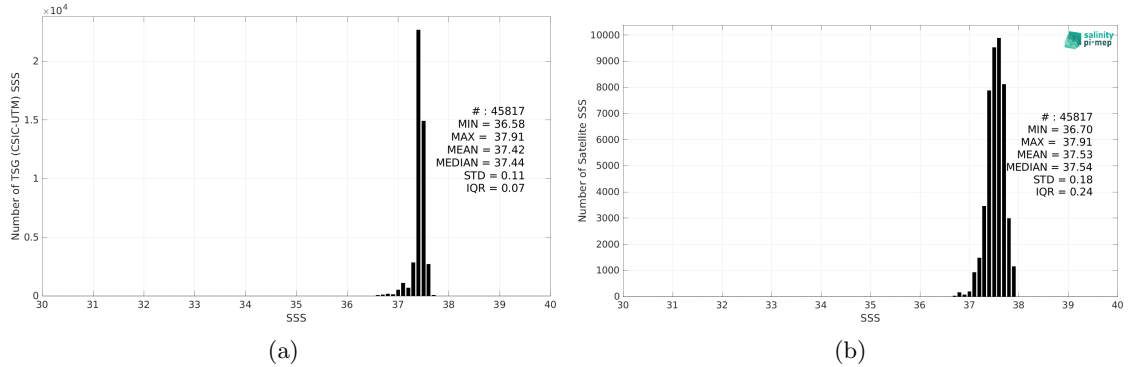
Figure 2: Histograms of SSS from TSG (CSIC-UTM) (a) and SMOS SSS L3 v8 - 9 Days (CATDS-CEC-LOCEAN) (b) considering all match-up pairs per bins of 0.1 over the SPURS 1 Pi-MEP region and for the full satellite product period.
