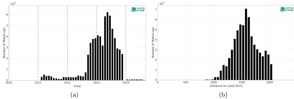
Figure 1: Number of match-ups between Surface drifters and SMOS SSS L3 v8 - 9 Days (CATDS-CEC-LOCEAN) SSS as a function of time (a) and as function of the distance to coast (b) over the SPURS 1 Pi-MEP region and for the full satellite product period.
