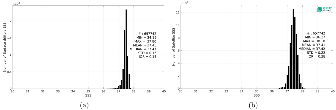
Figure 2: Histograms of SSS from Surface drifters (a) and SMOS SSS L3 v8 - 9 Days (CATDS-CEC-LOCEAN) (b) considering all match-up pairs per bins of 0.1 over the SPURS 1 Pi-MEP region and for the full satellite product period.
