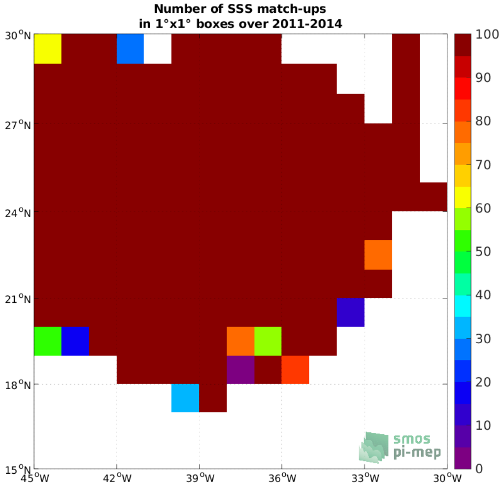
Figure 3: Number of SSS match-ups between Surface drifters SSS and the SMOS SSS L3 v8 - 9 Days (CATDS-CECOS-LOCEAN) SSS product for the SPURS 1 Pi-MEP region over 1°x1° boxes and for the full satellite product period.
