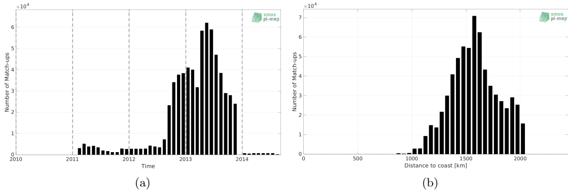
Figure 1: Number of match-ups between Surface drifters and SMOS SSS L3 v8 - 9 Days (CATDS-CECOS-LOCEAN) SSS as a function of time (a) and as function of the distance to coast (b) over the SPURS 1 Pi-MEP region and for the full satellite product period.
