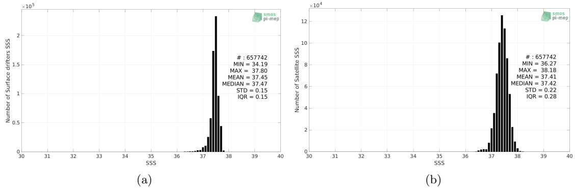
Figure 2: Histograms of SSS from Surface drifters (a) and SMOS SSS L3 v8 - 9 Days (CATDS-CECOS-LOCEAN) (b) considering all match-up pairs per bins of 0.1 over the SPURS 1 Pi-MEP region and for the full satellite product period.
