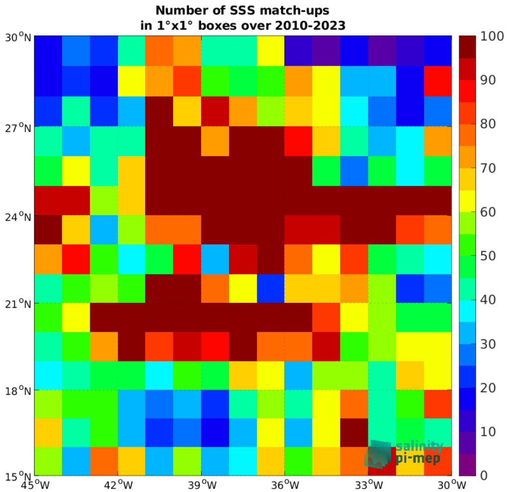
Figure 4: Number of SSS match-ups between Argo SSS and the SMOS SSS L3 v8 - 9 Days (CATDS-CEC-LOCEAN) SSS product for the SPURS 1 Pi-MEP region over 1°x1° boxes and for the full satellite product period.
