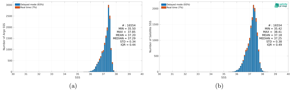
Figure 2: Histograms of SSS from Argo (a) and SMOS SSS L3 v8 - 9 Days (CATDS-CEC-LOCEAN) (b) considering all match-up pairs per bins of 0.1 over the SPURS 1 Pi-MEP region and for the full satellite product period.
