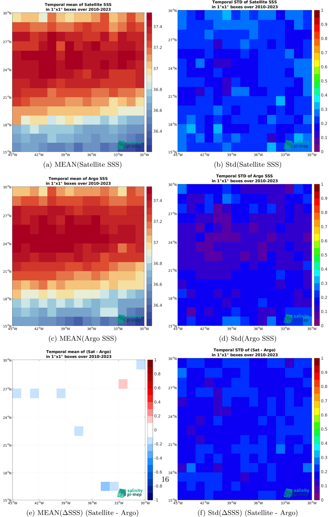
Figure 6: Temporal mean (left) and Std (right) of SSS from SMOS SSS L3 v8 - 9 Days (CATDS-CEC-LOCEAN) (top), Argo (middle), and of \Delta SSS (Satellite - Argo). Only match-up pairs are used to generate these maps.
