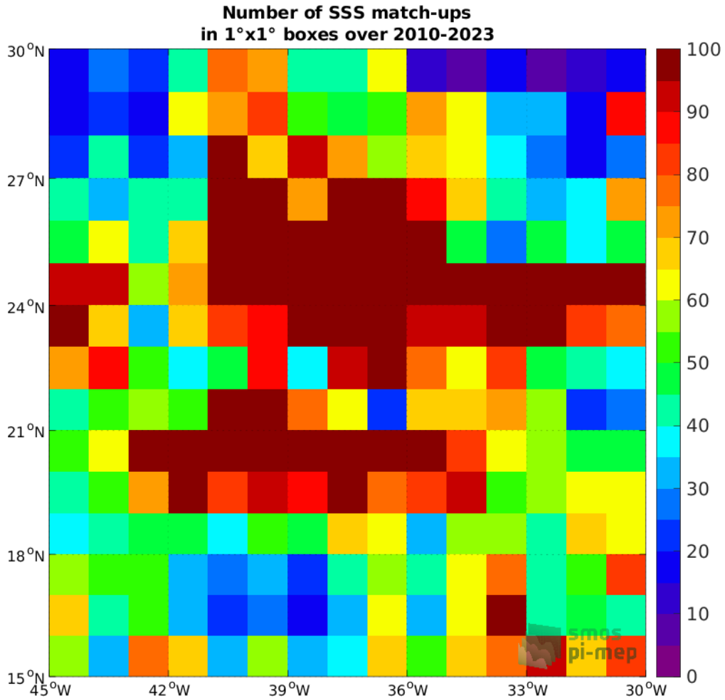
Figure 4: Number of SSS match-ups between Argo SSS and the SMOS SSS L3 v8 - 9 Days (CATDS-CECOS-LOCEAN) SSS product for the SPURS 1 Pi-MEP region over 1°x1° boxes and for the full satellite product period.
