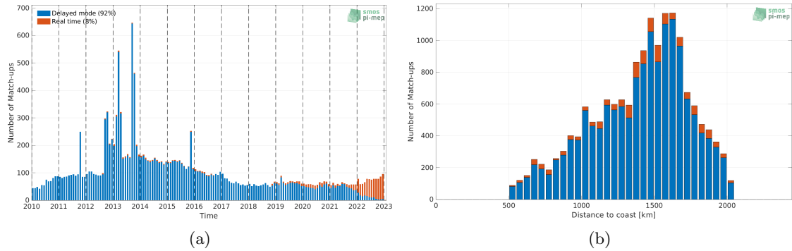
Figure 1: Number of match-ups between Argo and SMOS SSS L3 v8 - 9 Days (CATDS-CECOS-LOCEAN) SSS as a function of time (a) and as function of the distance to coast (b) over the SPURS 1 Pi-MEP region and for the full satellite product period.
