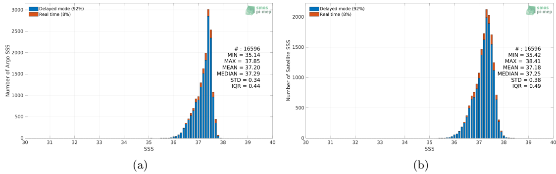
Figure 2: Histograms of SSS from Argo (a) and SMOS SSS L3 v8 - 9 Days (CATDS-CECOS-LOCEAN) (b) considering all match-up pairs per bins of 0.1 over the SPURS 1 Pi-MEP region and for the full satellite product period.
