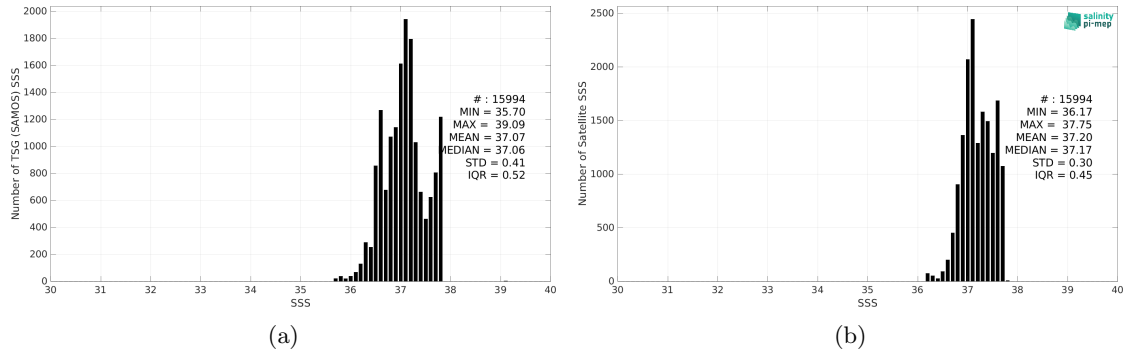
Figure 2: Histograms of SSS from TSG (SAMOS) (a) and SMOS SSS L3 v8 - 18 Days (CATDS-CEC-LOCEAN) (b) considering all match-up pairs per bins of 0.1 over the SPURS 1 Pi-MEP region and for the full satellite product period.
