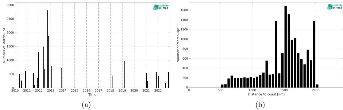
Figure 1: Number of match-ups between TSG (SAMOS) and SMOS SSS L3 v8 - 18 Days (CATDS-CEC-LOCEAN) SSS as a function of time (a) and as function of the distance to coast (b) over the SPURS 1 Pi-MEP region and for the full satellite product period.
