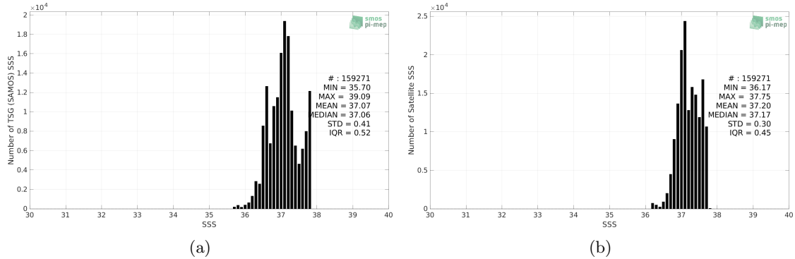
Figure 2: Histograms of SSS from TSG (SAMOS) (a) and SMOS SSS L3 v8 - 18 Days (CATDS-CECOS-LOCEAN) (b) considering all match-up pairs per bins of 0.1 over the SPURS 1 Pi-MEP region and for the full satellite product period.
