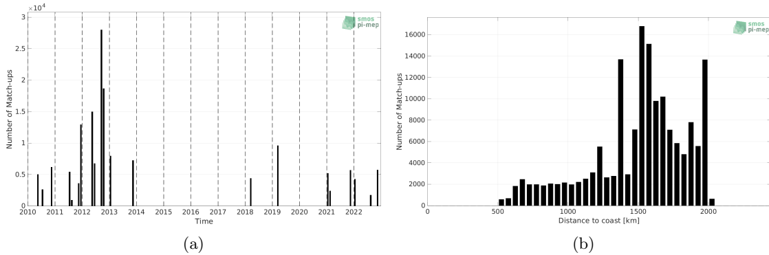
Figure 1: Number of match-ups between TSG (SAMOS) and SMOS SSS L3 v8 - 18 Days (CATDS-CECOS-LOCEAN) SSS as a function of time (a) and as function of the distance to coast (b) over the SPURS 1 Pi-MEP region and for the full satellite product period.
