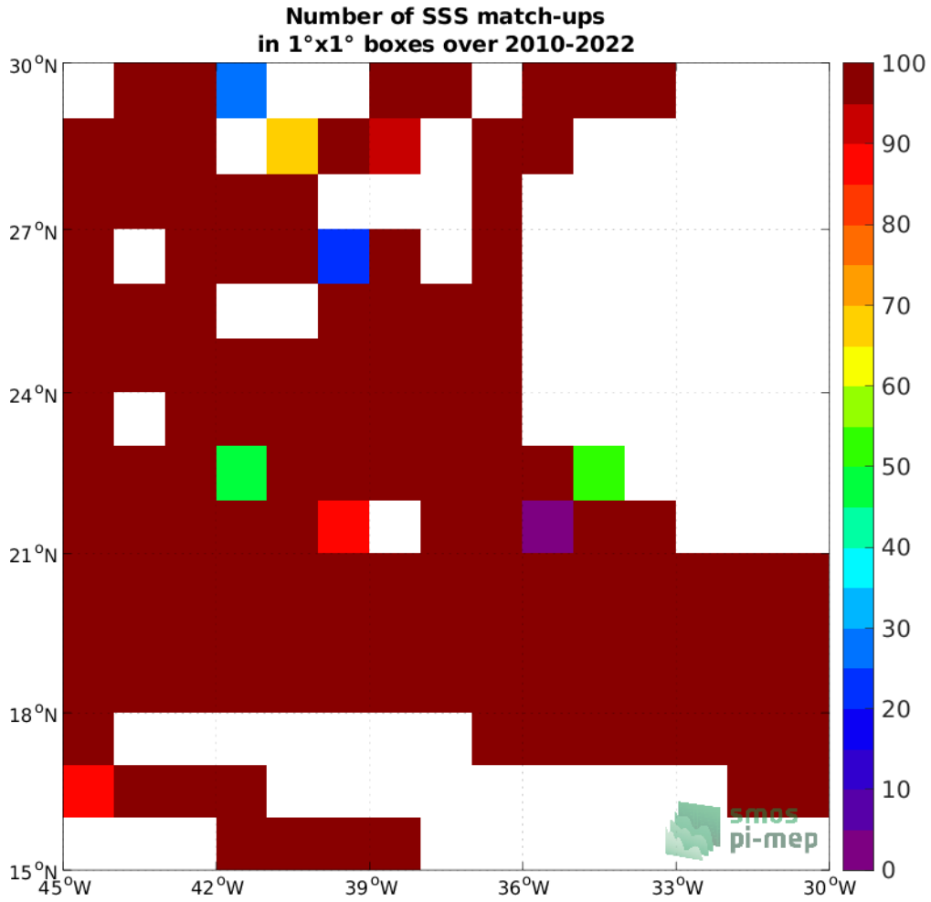
Figure 4: Number of SSS match-ups between TSG (SAMOS) SSS and the SMOS SSS L3 v8 - 18 Days (CATDS-CECOS-LOCEAN) SSS product for the SPURS 1 Pi-MEP region over 1°x1° boxes and for the full satellite product period.
