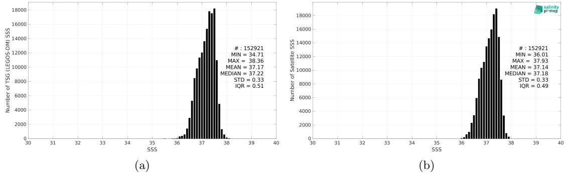
Figure 2: Histograms of SSS from TSG (LEGOS-DM) (a) and SMOS SSS L3 v8 - 18 Days (CATDS-CEC-LOCEAN) (b) considering all match-up pairs per bins of 0.1 over the SPURS 1 Pi-MEP region and for the full satellite product period.
