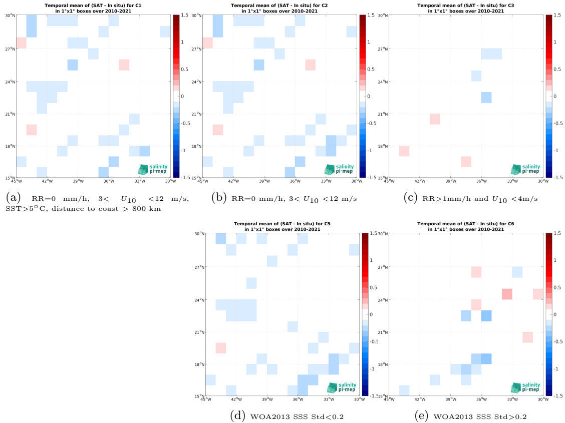
Figure 12: Temporal mean gridded over spatial boxes of size 1^{\circ}\times 1^{\circ} of \Delta\text{SSS} (SMOS SSS L3 v8 - 18 Days (CATDS-CEC-LOCEAN) - TSG (LEGOS-DM)) for 5 different subdatasets corresponding to:RR=0 mm/h, 3 < U_{10} < 12 m/s, SST >5^{\circ}\text{C} , distance to coast > 800 km (a), RR=0 mm/h, 3 < U_{10} < 12 m/s (b), RR >1 mm/h and U_{10} < 4 m/s (c), WOA2013 SSS Std <0.2 (d), WOA2013 SSS Std >0.2 (e).
