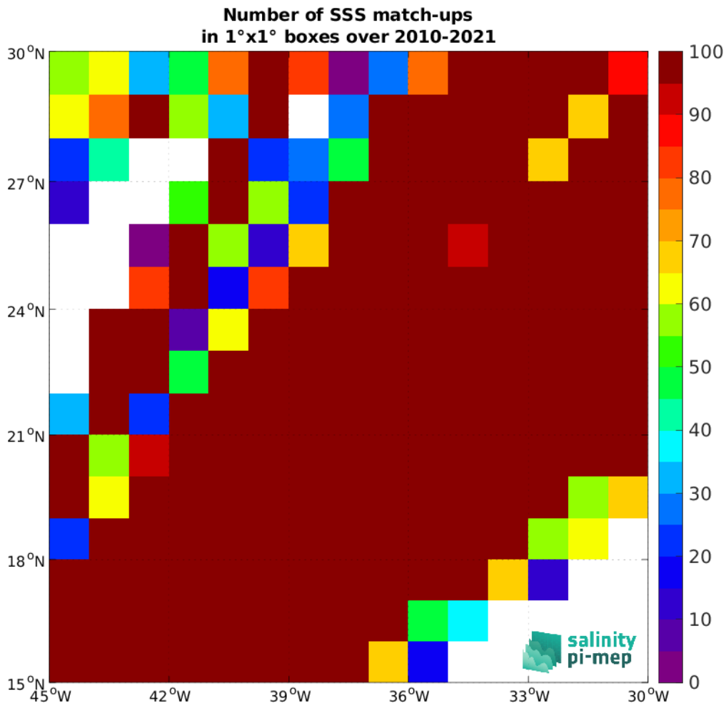
Figure 4: Number of SSS match-ups between TSG (LEGOS-DM) SSS and the SMOS SSS L3 v8 - 18 Days (CATDS-CEC-LOCEAN) SSS product for the SPURS 1 Pi-MEP region over 1°x1° boxes and for the full satellite product period.
