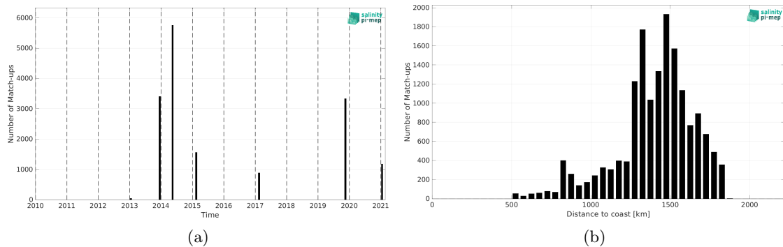
Figure 1: Number of match-ups between TSG (GOSUD-Sailing-ship) and SMOS SSS L3 v8 - 18 Days (CATDS-CEC-LOCEAN) SSS as a function of time (a) and as function of the distance to coast (b) over the SPURS 1 Pi-MEP region and for the full satellite product period.
