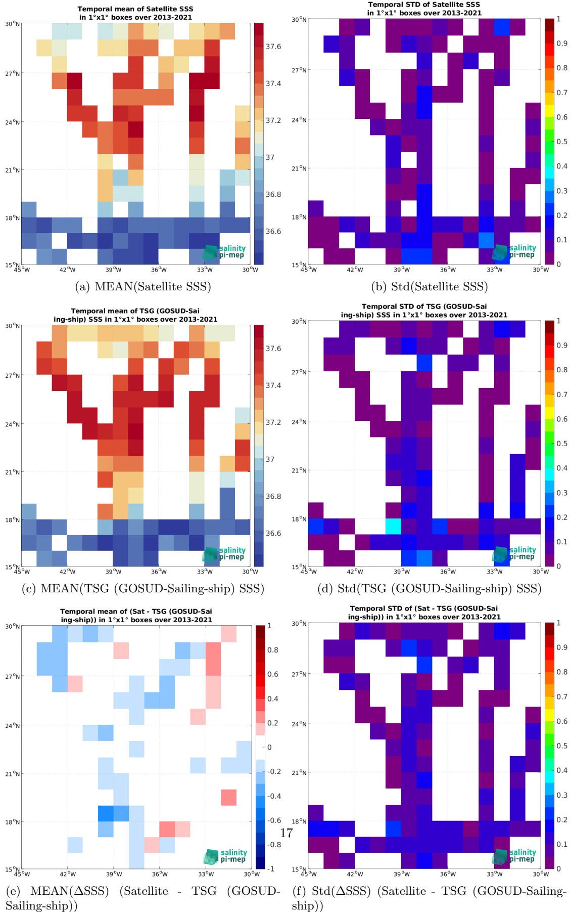
Figure 6: Temporal mean (left) and Std (right) of SSS from SMOS SSS L3 v8 - 18 Days (CATDS-CEC-LOCEAN) (top), TSG (GOSUD-Sailing-ship) (middle), and of \Delta SSS (Satellite - TSG (GOSUD-Sailing-ship)). Only match-up pairs are used to generate these maps.
