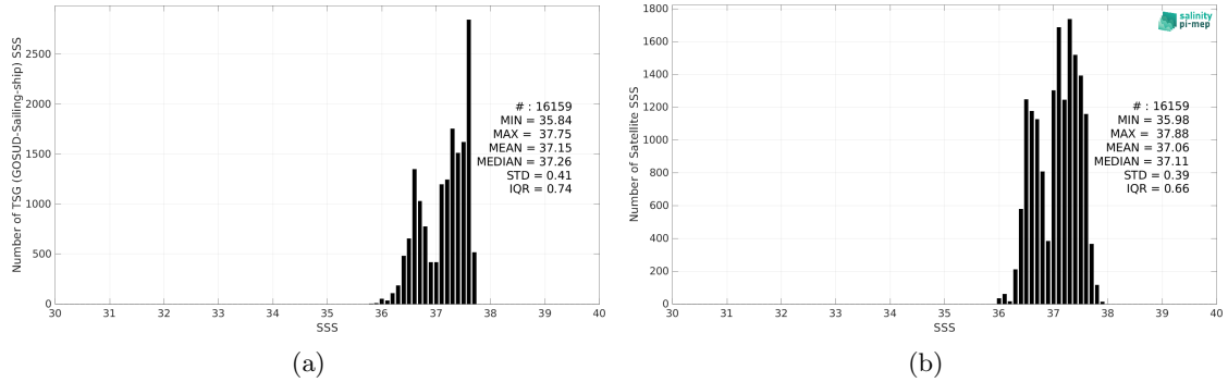
Figure 2: Histograms of SSS from TSG (GOSUD-Sailing-ship) (a) and SMOS SSS L3 v8 - 18 Days (CATDS-CEC-LOCEAN) (b) considering all match-up pairs per bins of 0.1 over the SPURS 1 Pi-MEP region and for the full satellite product period.
