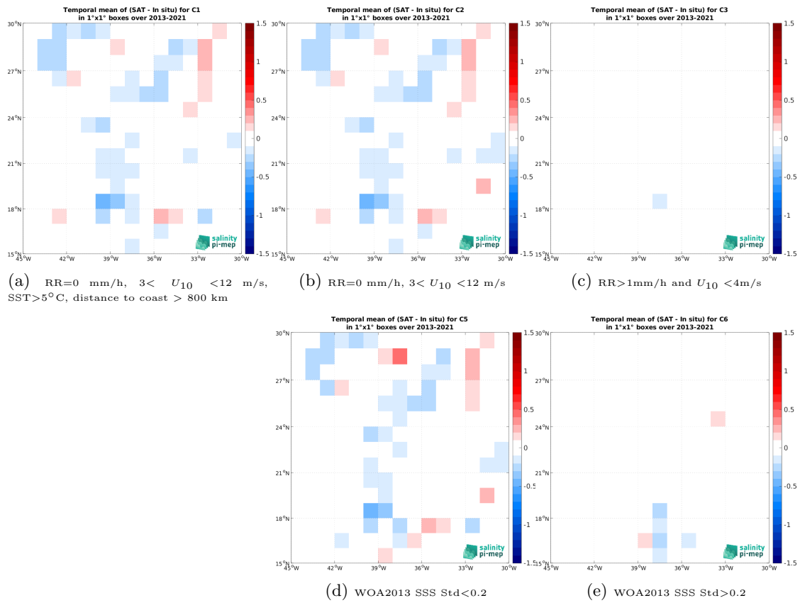
Figure 12: Temporal mean gridded over spatial boxes of size 1^{\circ} \times 1^{\circ} of \Delta\text{SSS} (SMOS SSS L3 v8 - 18 Days (CATDS-CEC-LOCEAN) - TSG (GOSUD-Sailing-ship)) for 5 different subdatasets corresponding to: RR=0 mm/h, 3 < U_{10} < 12 m/s, SST > 5^{\circ}\text{C} , distance to coast > 800 km (a), RR=0 mm/h, 3 < U_{10} < 12 m/s (b), RR > 1\text{mm/h} and U_{10} < 4\text{m/s} (c), WOA2013 SSS Std < 0.2 (d), WOA2013 SSS Std > 0.2 (e).
