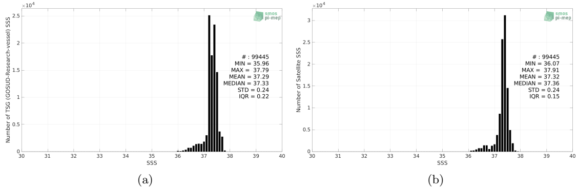
Figure 2: Histograms of SSS from TSG (GOSUD-Research-vessel) (a) and SMOS SSS L3 v8 - 18 Days (CATDS-CECOS-LOCEAN) (b) considering all match-up pairs per bins of 0.1 over the SPURS 1 Pi-MEP region and for the full satellite product period.
