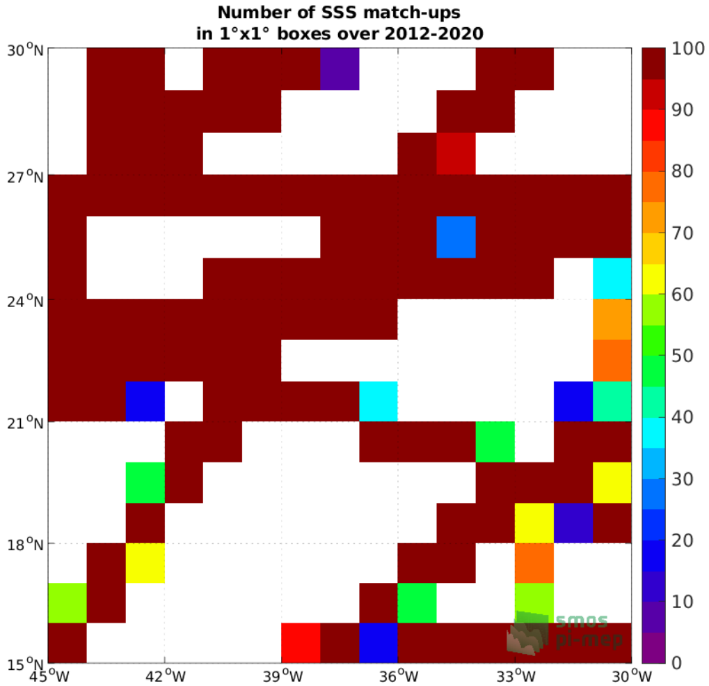
Figure 4: Number of SSS match-ups between TSG (GOSUD-Research-vessel) SSS and the SMOS SSS L3 v8 - 18 Days (CATDS-CECOS-LOCEAN) SSS product for the SPURS 1 Pi-MEP region over 1°x1° boxes and for the full satellite product period.
