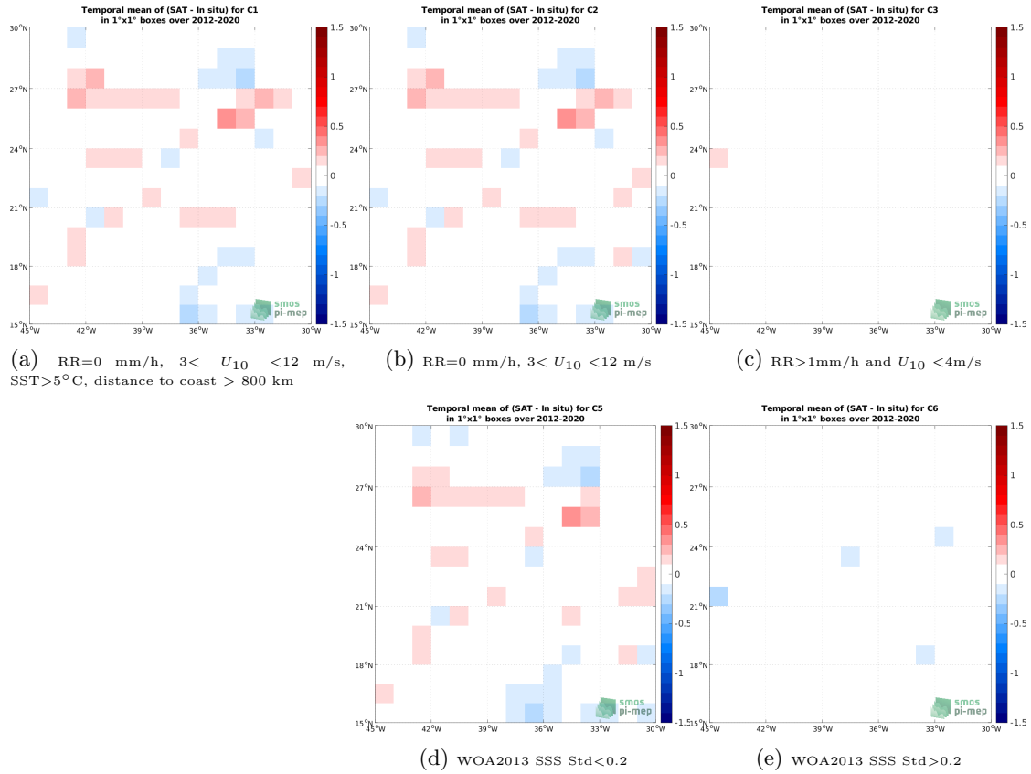
Figure 12: Temporal mean gridded over spatial boxes of size 1^\circ \times 1^\circ of \Delta SSS (SMOS SSS L3 v8 - 18 Days (CATDS-CECOS-LOCEAN) - TSG (GOSUD-Research-vessel)) for 5 different sub-datasets corresponding to: RR=0 mm/h, 3 < U_{10} < 12 m/s, SST > 5°C, distance to coast > 800 km (a), RR=0 mm/h, 3 < U_{10} < 12 m/s (b), RR > 1mm/h and U_{10} < 4 m/s (c), WOA2013 SSS Std < 0.2 (d), WOA2013 SSS Std > 0.2 (e).
