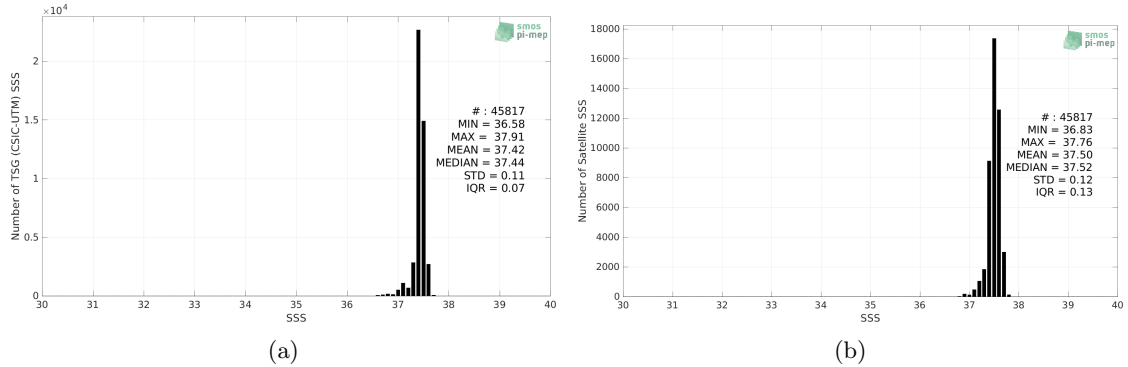
Figure 2: Histograms of SSS from TSG (CSIC-UTM) (a) and SMOS SSS L3 v8 - 18 Days (CATDS-CECOS-LOCEAN) (b) considering all match-up pairs per bins of 0.1 over the SPURS 1 Pi-MEP region and for the full satellite product period.
