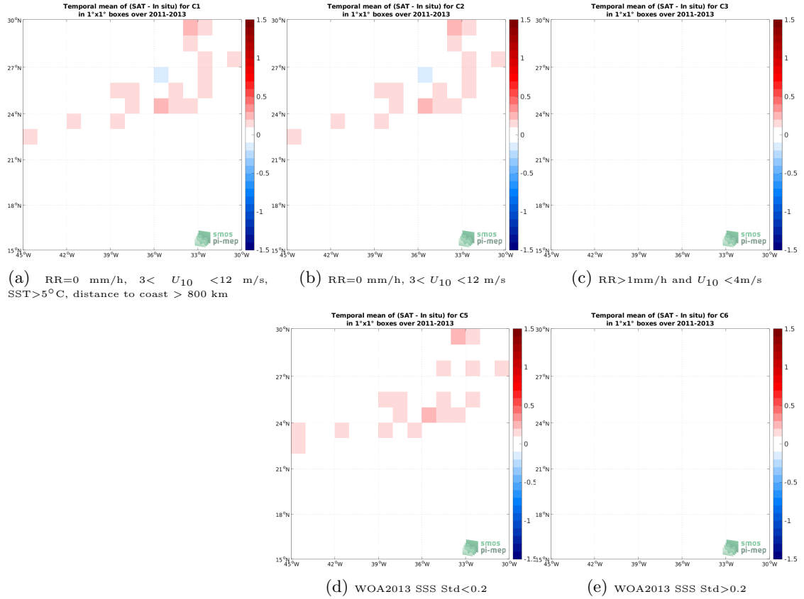
Figure 12: Temporal mean gridded over spatial boxes of size 1^{\circ}\times 1^{\circ} of \Delta\text{SSS} (SMOS SSS L3 v8 - 18 Days (CATDS-CECOS-LOCEAN) - TSG (CSIC-UTM)) for 5 different subdatasets corresponding to:RR=0 mm/h, 3 < U_{10} < 12 m/s, SST >5^{\circ}\text{C} , distance to coast > 800 km (a), RR=0 mm/h, 3 < U_{10} < 12 m/s (b), RR >1 mm/h and U_{10} < 4 m/s (c), WOA2013 SSS Std <0.2 (d), WOA2013 SSS Std >0.2 (e).
