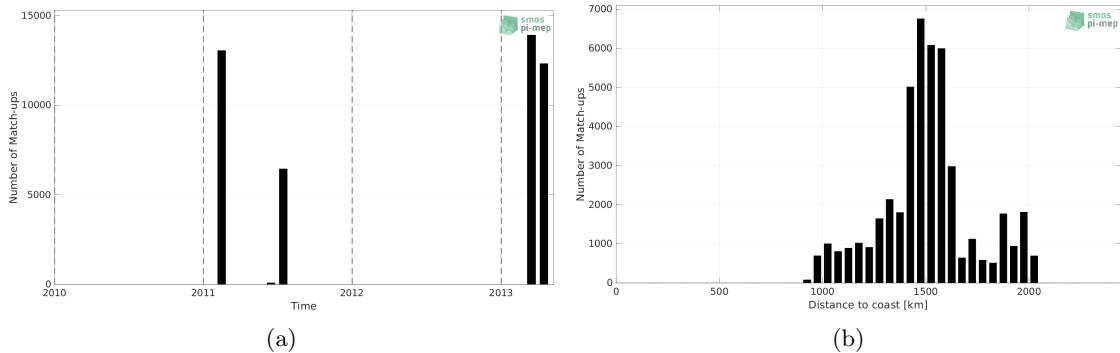
Figure 1: Number of match-ups between TSG (CSIC-UTM) and SMOS SSS L3 v8 - 18 Days (CATDS-CECOS-LOCEAN) SSS as a function of time (a) and as function of the distance to coast (b) over the SPURS 1 Pi-MEP region and for the full satellite product period.
