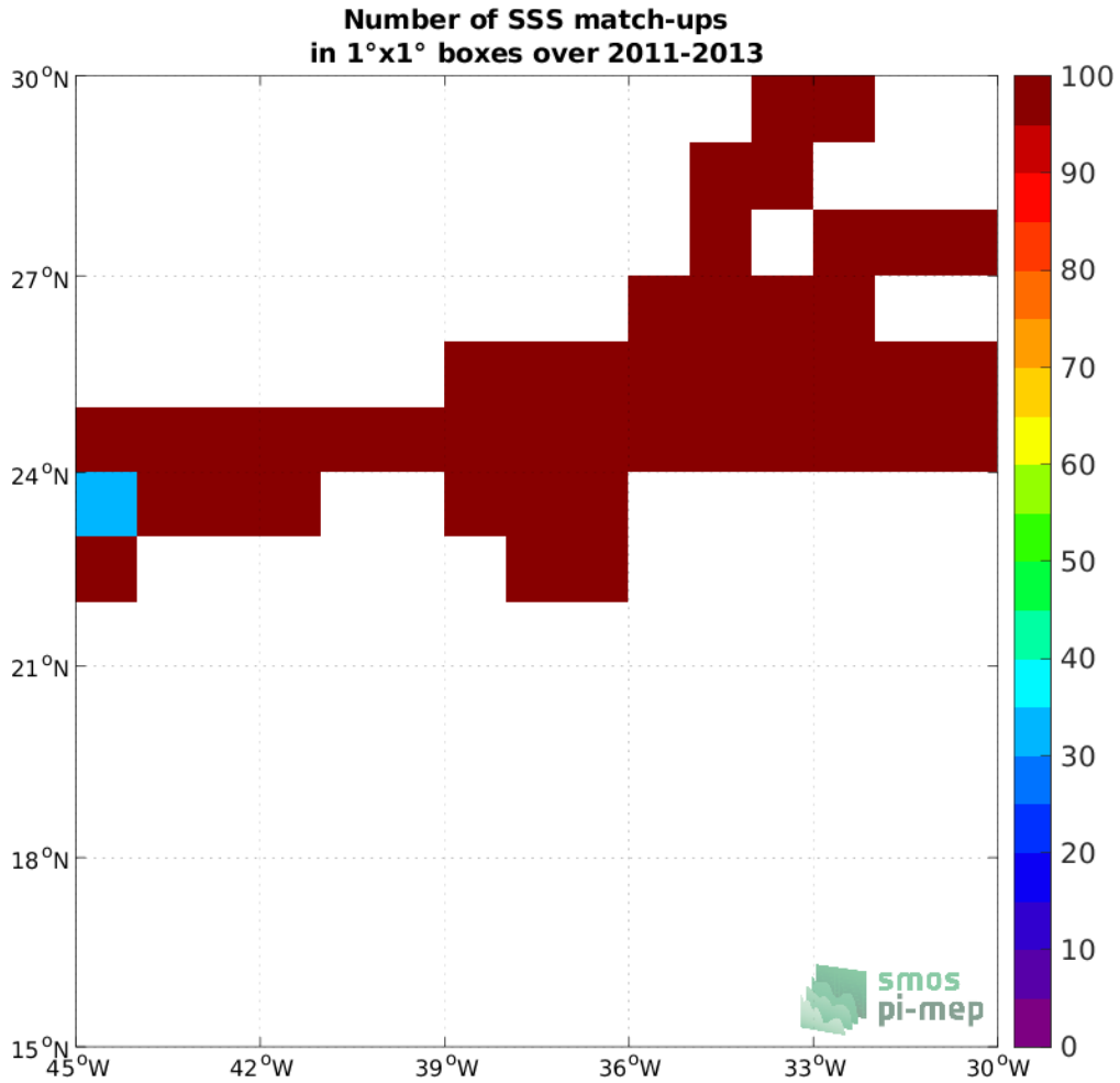
Figure 4: Number of SSS match-ups between TSG (CSIC-UTM) SSS and the SMOS SSS L3 v8 - 18 Days (CATDS-CECOS-LOCEAN) SSS product for the SPURS 1 Pi-MEP region over 1°x1° boxes and for the full satellite product period.
