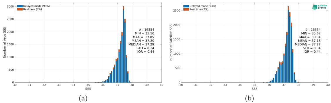
Figure 2: Histograms of SSS from Argo (a) and SMOS SSS L3 v8 - 18 Days (CATDS-CEC-LOCEAN) (b) considering all match-up pairs per bins of 0.1 over the SPURS 1 Pi-MEP region and for the full satellite product period.
