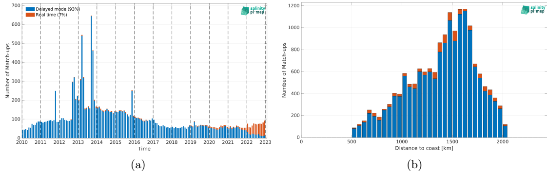
Figure 1: Number of match-ups between Argo and SMOS SSS L3 v8 - 18 Days (CATDS-CEC-LOCEAN) SSS as a function of time (a) and as function of the distance to coast (b) over the SPURS 1 Pi-MEP region and for the full satellite product period.
