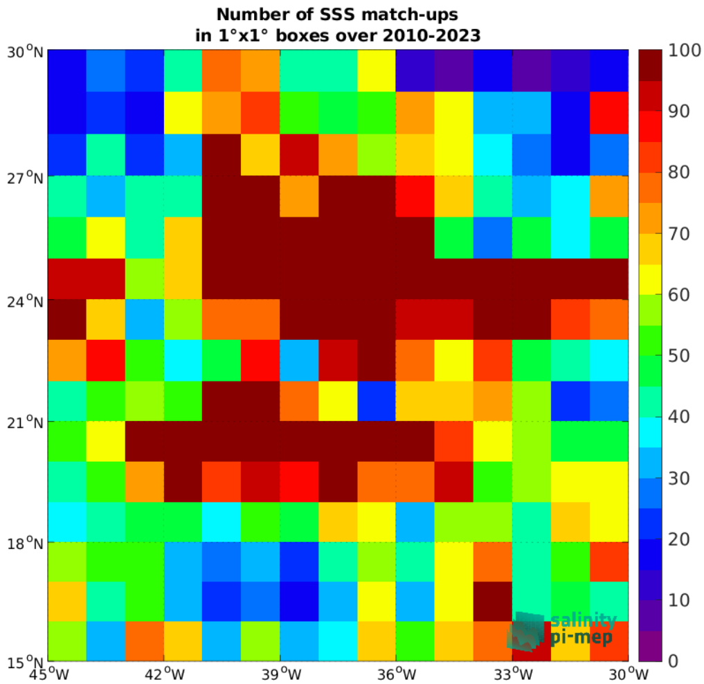
Figure 4: Number of SSS match-ups between Argo SSS and the SMOS SSS L3 v8 - 18 Days (CATDS-CEC-LOCEAN) SSS product for the SPURS 1 Pi-MEP region over 1°×1° boxes and for the full satellite product period.
