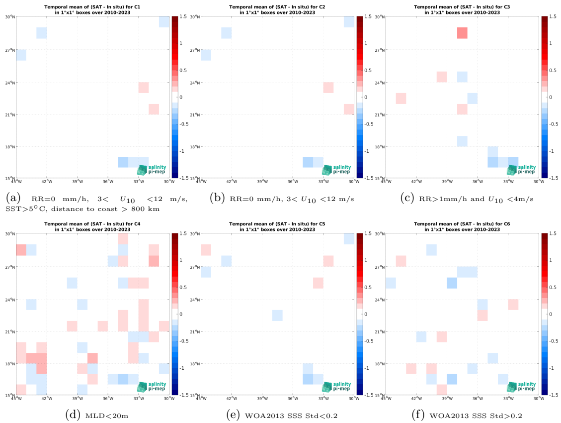
Figure 12: Temporal mean gridded over spatial boxes of size 1^\circ \times 1^\circ of \Delta SSS (SMOS SSS L3 v8 - 18 Days (CATDS-CEC-LOCEAN) - Argo) for 6 different subdatasets corresponding to:RR=0 mm/h, 3 < U_{10} < 12 m/s, SST >5^\circ\text{C} , distance to coast > 800 km (a), RR=0 mm/h, 3 < U_{10} < 12 m/s (b), RR >1 mm/h and U_{10} < 4 m/s (c),MLD <20 m (d),WOA2013 SSS Std <0.2 (e),WOA2013 SSS Std >0.2 (f).
