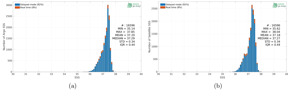
Figure 2: Histograms of SSS from Argo (a) and SMOS SSS L3 v8 - 18 Days (CATDS-CECOS-LOCEAN) (b) considering all match-up pairs per bins of 0.1 over the SPURS 1 Pi-MEP region and for the full satellite product period.
