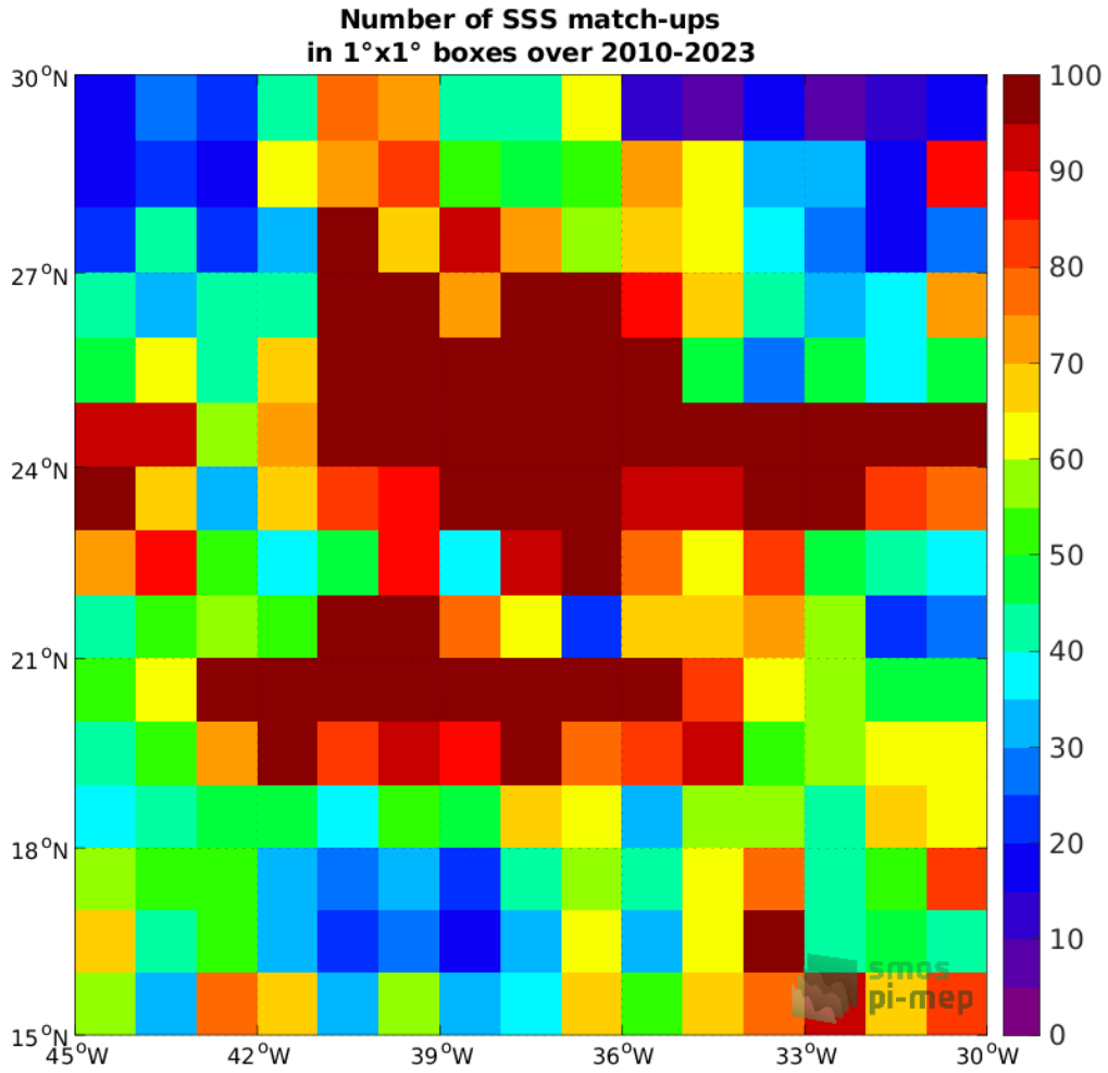
Figure 4: Number of SSS match-ups between Argo SSS and the SMOS SSS L3 v8 - 18 Days (CATDS-CECOS-LOCEAN) SSS product for the SPURS 1 Pi-MEP region over 1°x1° boxes and for the full satellite product period.
