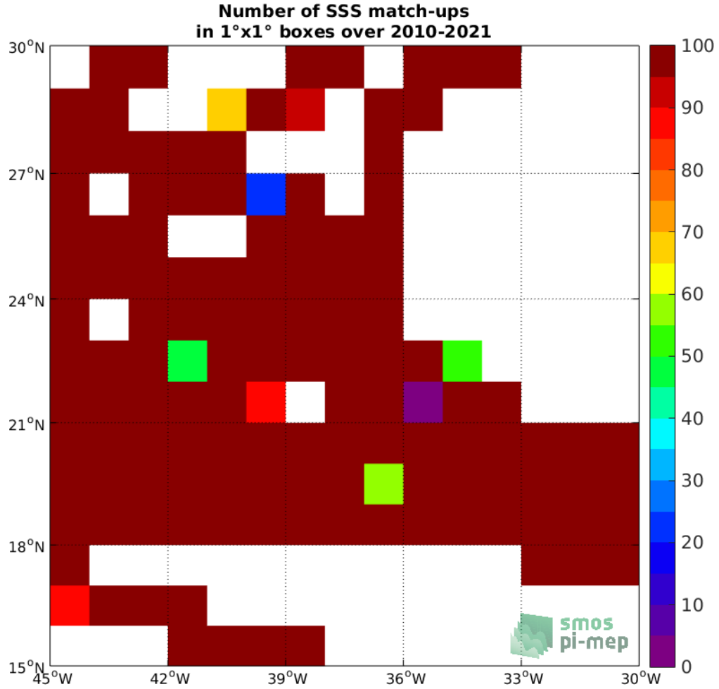
Figure 4: Number of SSS match-ups between TSG (SAMOS) SSS and the SMOS SSS L3 v7 - 9 Days (CATDS-CECOS-LOCEAN) SSS product for the SPURS 1 Pi-MEP region over 1^\circ \times 1^\circ boxes and for the full satellite product period.
