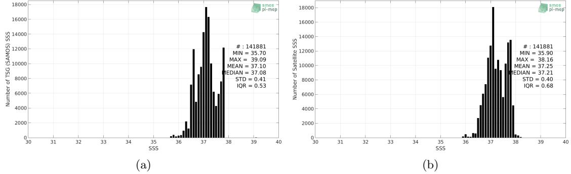
Figure 2: Histograms of SSS from TSG (SAMOS) (a) and SMOS SSS L3 v7 - 9 Days (CATDS-CECOS-LOCEAN) (b) considering all match-up pairs per bins of 0.1 over the SPURS 1 Pi-MEP region and for the full satellite product period.
