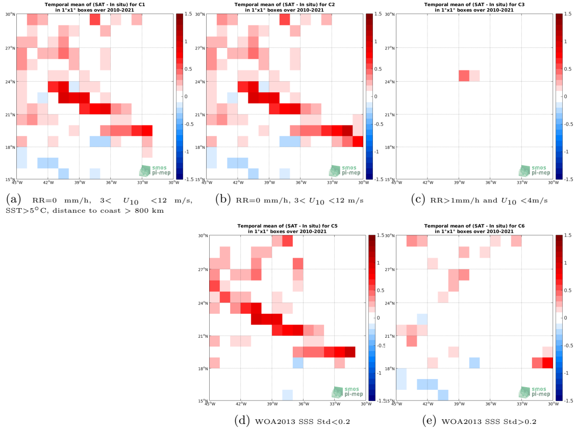
Figure 12: Temporal mean gridded over spatial boxes of size 1^{\circ}\times 1^{\circ} of \Delta\text{SSS} (SMOS SSS L3 v7 - 9 Days (CATDS-CECOS-LOCEAN) - TSG (SAMOS)) for 5 different subdatasets corresponding to: RR=0 mm/h, 3 < U_{10} < 12 m/s, SST >5^{\circ}\text{C} , distance to coast > 800 km (a), RR=0 mm/h, 3 < U_{10} < 12 m/s (b), RR >1 mm/h and U_{10} < 4 m/s (c), WOA2013 SSS Std <0.2 (d), WOA2013 SSS Std >0.2 (e).
