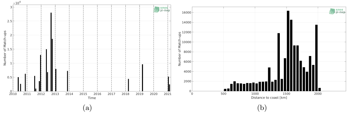
Figure 1: Number of match-ups between TSG (SAMOS) and SMOS SSS L3 v7 - 9 Days (CATDS-CECOS-LOCEAN) SSS as a function of time (a) and as function of the distance to coast (b) over the SPURS 1 Pi-MEP region and for the full satellite product period.
