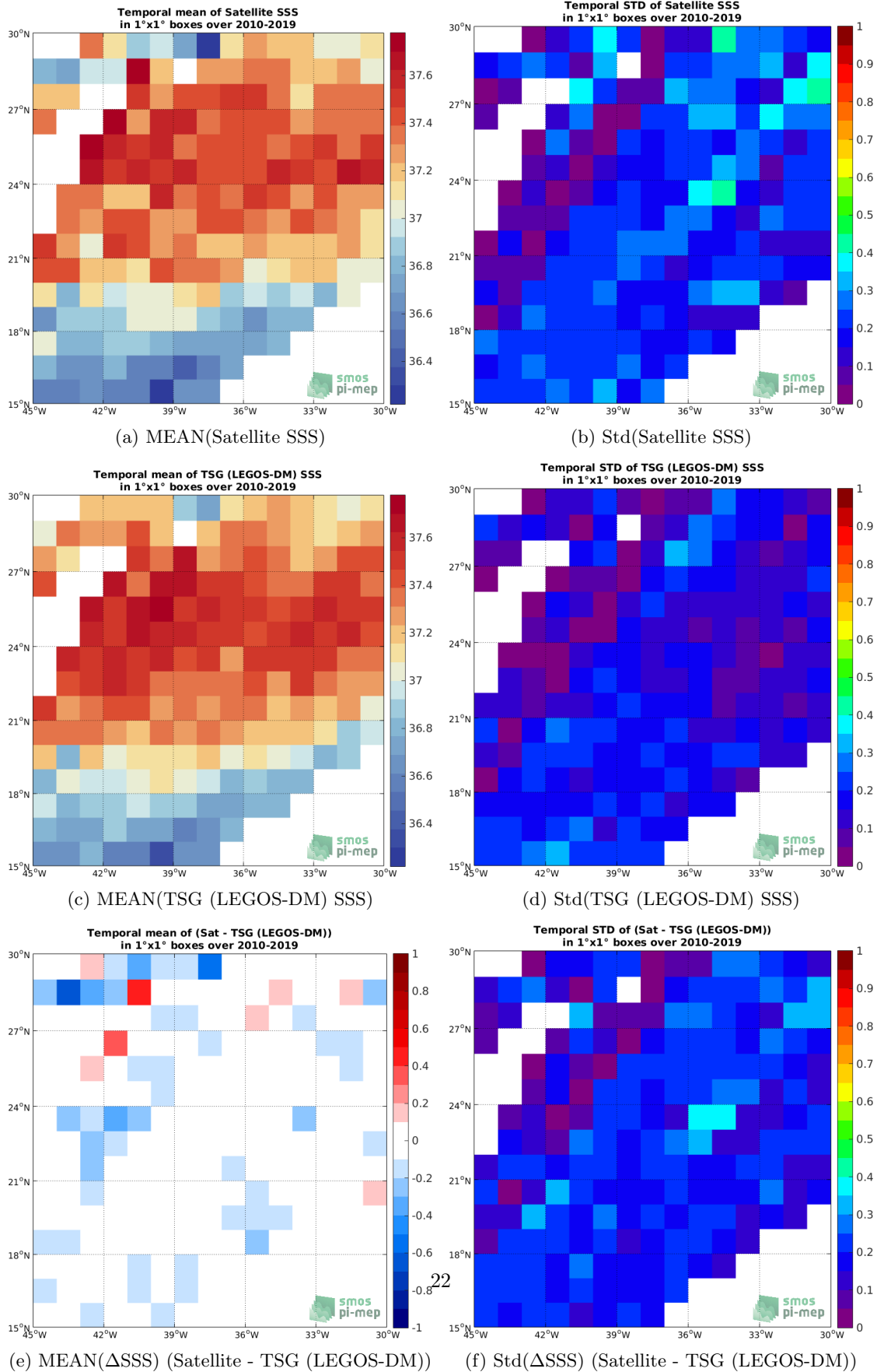
Figure 6: Temporal mean (left) and Std (right) of SSS from SMOS SSS L3 v7 - 9 Days (CATDS-CECOS-LOCEAN) (top), TSG (LEGOS-DM) (middle), and of \Delta SSS (Satellite - TSG (LEGOS-DM)). Only match-up pairs are used to generate these maps.
