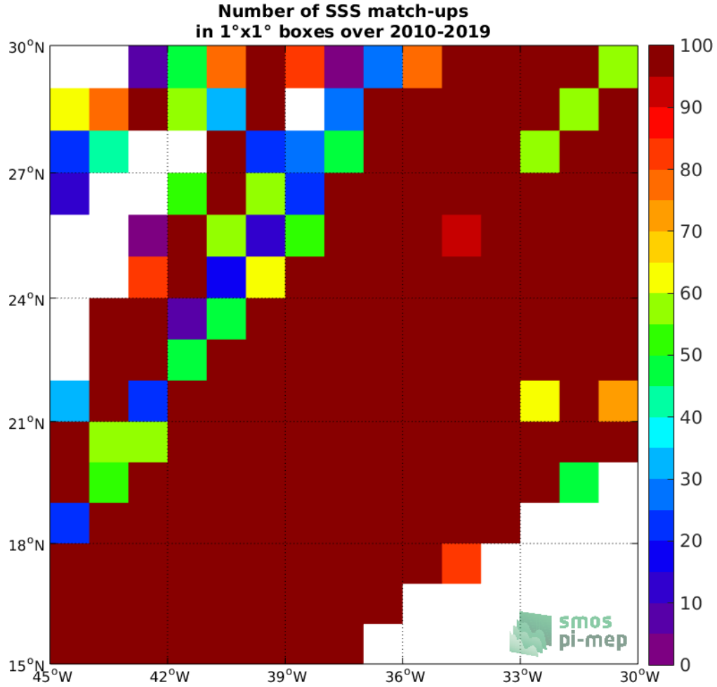
Figure 4: Number of SSS match-ups between TSG (LEGOS-DM) SSS and the SMOS SSS L3 v7 - 9 Days (CATDS-CECOS-LOCEAN) SSS product for the SPURS 1 Pi-MEP region over 1^\circ \times 1^\circ boxes and for the full satellite product period.
