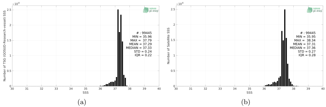
Figure 2: Histograms of SSS from TSG (GOSUD-Research-vessel) (a) and SMOS SSS L3 v7 - 9 Days (CATDS-CECOS-LOCEAN) (b) considering all match-up pairs per bins of 0.1 over the SPURS 1 Pi-MEP region and for the full satellite product period.
