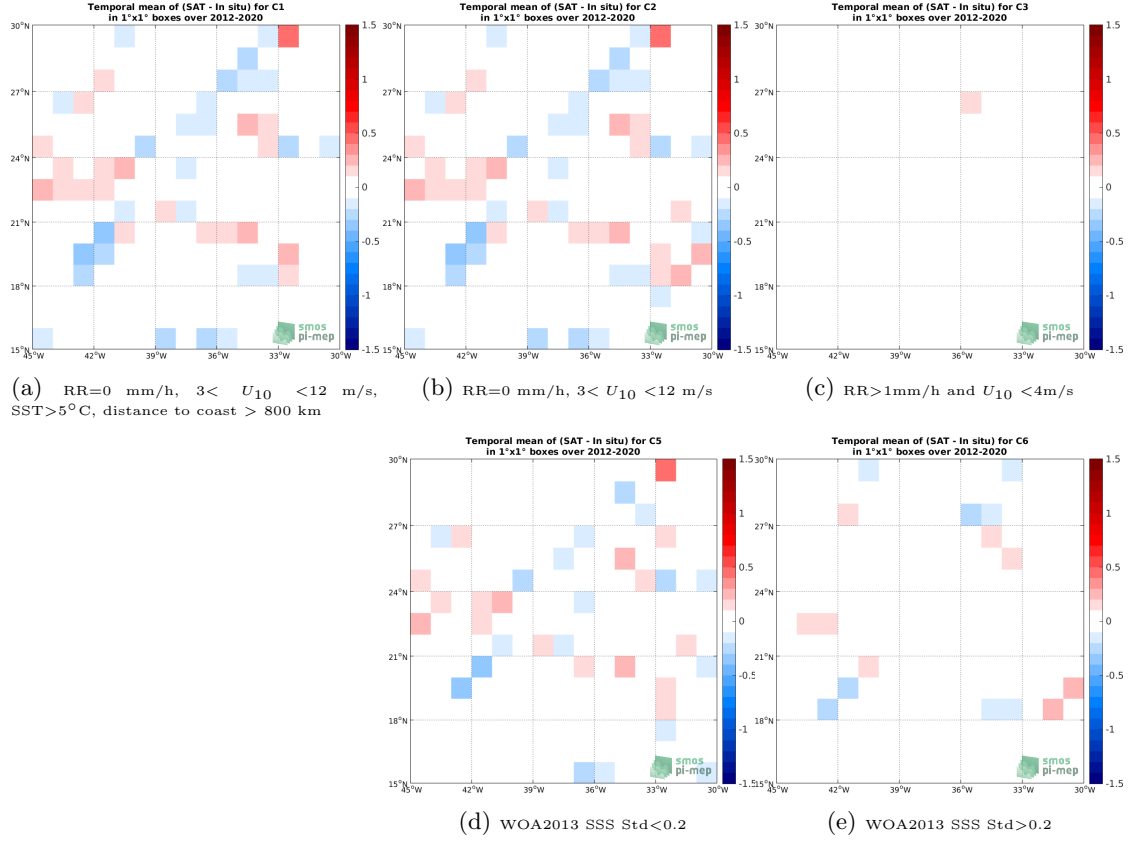
Figure 12: Temporal mean gridded over spatial boxes of size 1^\circ \times 1^\circ of \Delta\text{SSS} (SMOS SSS L3 v7 - 9 Days (CATDS-CECOS-LOCEAN) - TSG (GOSUD-Research-vessel)) for 5 different subdatasets corresponding to: RR=0 mm/h, 3 < U_{10} < 12 m/s, SST > 5^\circ\text{C} , distance to coast > 800 km (a), RR=0 mm/h, 3 < U_{10} < 12 m/s (b), RR > 1 mm/h and U_{10} < 4 m/s (c), WOA2013 SSS Std < 0.2 (d), WOA2013 SSS Std > 0.2 (e).
