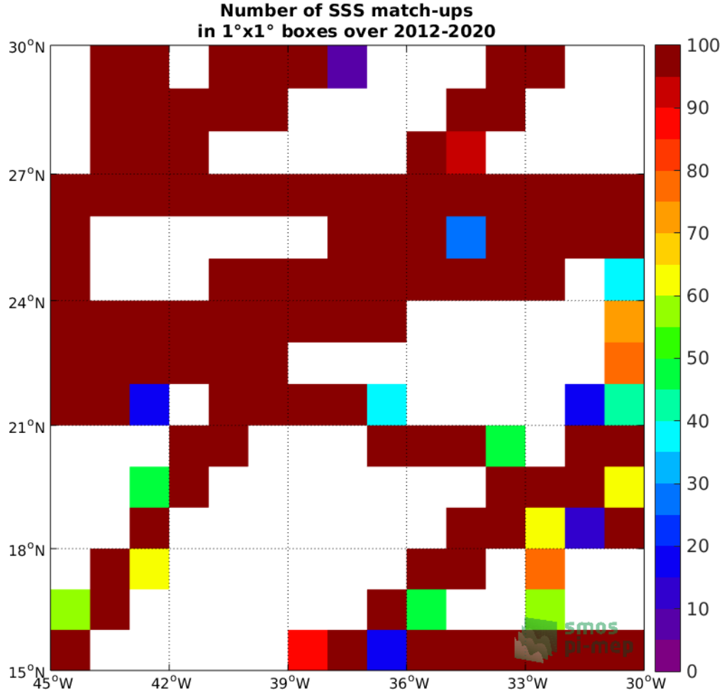
Figure 4: Number of SSS match-ups between TSG (GOSUD-Research-vessel) SSS and the SMOS SSS L3 v7 - 9 Days (CATDS-CECOS-LOCEAN) SSS product for the SPURS 1 Pi-MEP region over 1^\circ \times 1^\circ boxes and for the full satellite product period.
