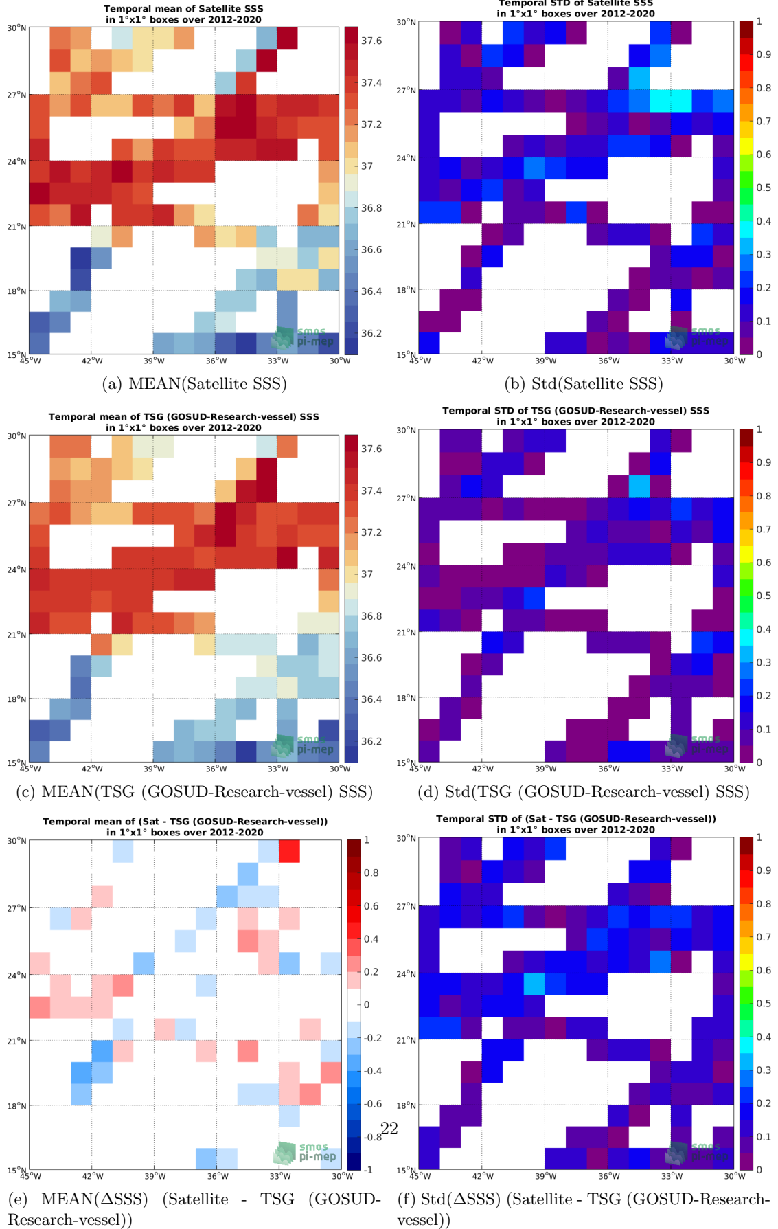
Figure 6: Temporal mean (left) and Std (right) of SSS from SMOS SSS L3 v7 - 9 Days (CATDS-CECOS-LOCEAN) (top), TSG (GOSUD-Research-vessel) (middle), and of \Delta SSS (Satellite - TSG (GOSUD-Research-vessel)). Only match-up pairs are used to generate these maps.
