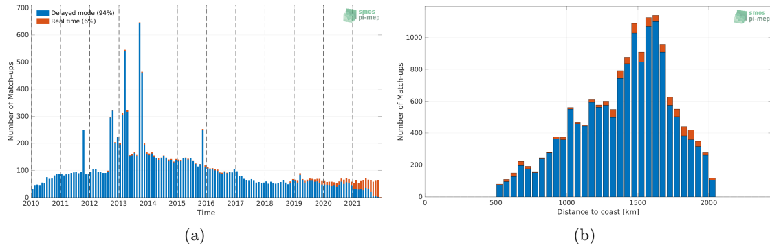
Figure 1: Number of match-ups between Argo and SMOS SSS L3 v7 - 9 Days (CATDS-CECOS-LOCEAN) SSS as a function of time (a) and as function of the distance to coast (b) over the SPURS 1 Pi-MEP region and for the full satellite product period.
