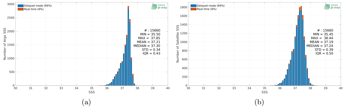
Figure 2: Histograms of SSS from Argo (a) and SMOS SSS L3 v7 - 9 Days (CATDS-CECOS-LOCEAN) (b) considering all match-up pairs per bins of 0.1 over the SPURS 1 Pi-MEP region and for the full satellite product period.
