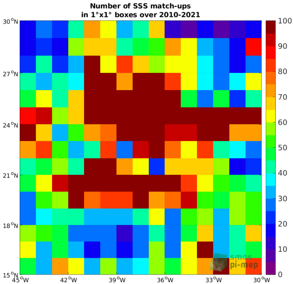
Figure 4: Number of SSS match-ups between Argo SSS and the SMOS SSS L3 v7 - 9 Days (CATDS-CECOS-LOCEAN) SSS product for the SPURS 1 Pi-MEP region over 1°x1° boxes and for the full satellite product period.
